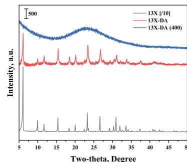
Fig. 1 XRD patterns of 13X and 13X-DA.
