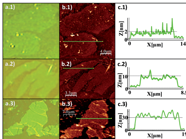
Fig. 2 Morphological characterization of layers of [\text{Cu}(\mu\text{-pym}_2\text{S}_2)(\mu\text{-Cl})]_n \cdot n\text{MeOH} on \text{SiO}_2 . Optical (a1–a3) and AFM topographic images (b1–b3) with their height profiles (c1–c3) showing thickness ranging from: single layer (2 nm, top), 14 layers (10 nm, middle) and 48 layers (30 nm, bottom).
