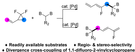
Scheme 1 Transition metal-catalyzed cross-coupling of gem -difluorinated cyclopropanes.
