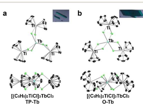
Fig. 1 (a) Molecular structure of TP-Tb with thermal ellipsoids at 50% probability. (Inset) Image of TP-Tb single crystals. (b) Molecular structure of O-Tb with thermal ellipsoids at 50% probability. (Inset) Image of O-Tb single crystals. Black, blue, green, and grey represent carbon, terbium, chlorine, and titanium, respectively.
