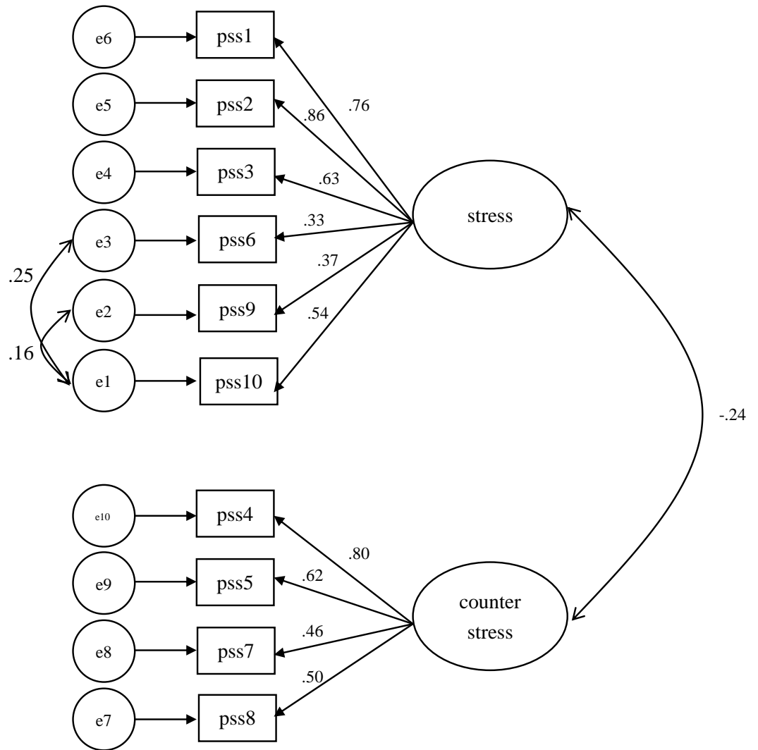
Figure 1 The two factors measurement model of the PSS-10.
