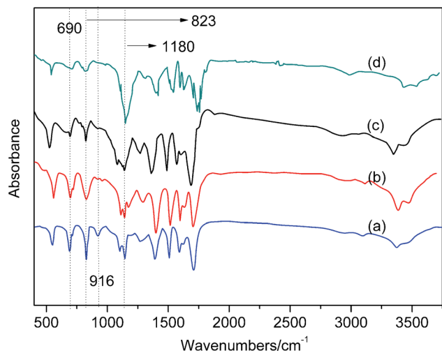
Fig. 8 FTIR spectra of 0.3 wt% AS-GO containing system as a function of sequential cure conditions: (a–d) at sequential temperature of 150 °C, 180 °C, 210 °C, 240 °C respectively.
