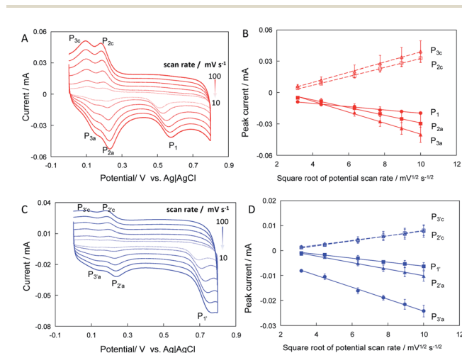
Fig. 4 CVs of CNT/Nafion/GC electrodes in phosphate buffer (pH 7.0 \pm 0.1 , 0.2 M) containing 0.1 mM hesperidin (A) and naringin (C) with potential scan rate varied from 10 to 100 \text{mV s}^{-1} , respectively. Relationships between peak current of CNT/Nafion/GC electrodes and square root of potential scan rate for hesperidin (B) and naringin (D).
