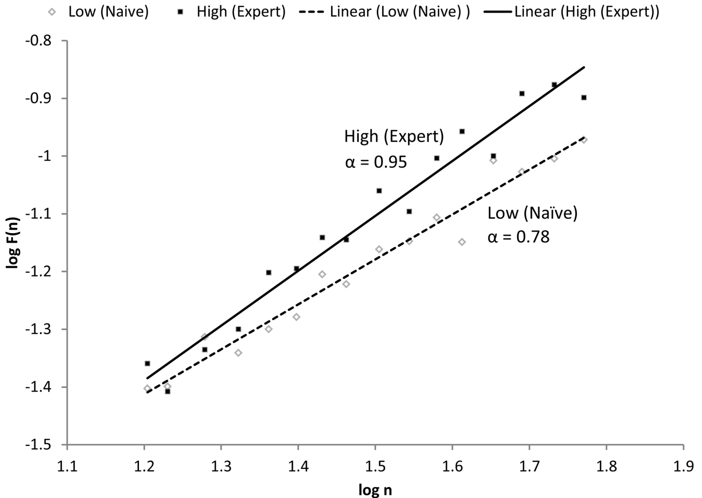
Fig 2. Example plots of a high (expert with \alpha = 0.95 ) and low (naïve with \alpha = 0.78 ) DFA alpha ( \alpha ) result. The slope of the linear best-fit line on the \log F(n) versus \log n plot represents alpha.
