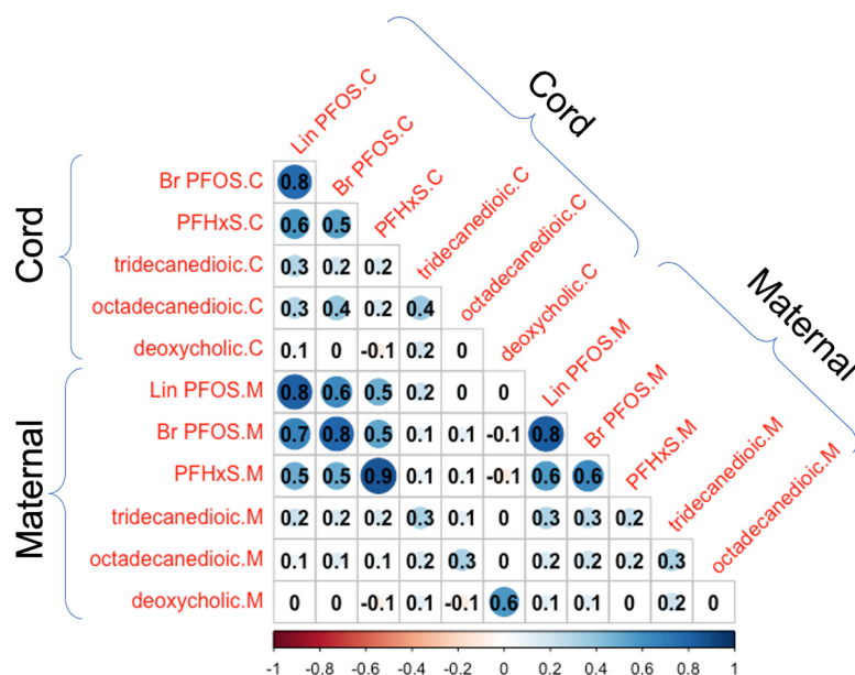
Figure 2. Spearman correlation coefficients for chemicals detected in maternal and cord serum samples, chemicals have at least 65% DF (maternal n = 302, cord n = 299). Chemical names ending in “M” refer to maternal samples, and “C” to cord blood samples. Note: Br, branched; DF, detection frequency; Lin, linear; PFHxS, perfluorohexane sulfonate; PFOS, perfluorooctane sulfonate.
