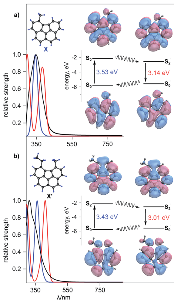
Fig. 4 (a) (Top left) Single-crystal X-ray structure of X. (Bottom left) Optical transition strengths computed at the ground state optimal geometry for X in THF (blue) and at the second singlet excited state optimal geometry for X in THF (red). (Right) Energies and isosurfaces of the HONTO and LUNTO of X in the ground and the second singlet excited states. S_0 and S_2 are the ground and excited states for X of the ground state. S_0' and S_2' are the ground and excited state intermediates for the minimum energy geometry of the second excited singlet state. The black solid and wavy arrows indicate absorption ( S_0 \rightarrow S_2 ) or emission ( S_2' \rightarrow S_0' ) and vibrational relaxation ( S_2 \rightarrow S_2' and S_2' \rightarrow S_2 ), respectively. The theory level is TDDFT/RPA based on the B3LYP-D3/6-31+G* method. (b) (Top left) Geometrically optimized structure of X' based on B3LYP-D3/6-31+G* level of theory. (Bottom left) Optical transition strengths computed at the ground state optimal geometry for X' in THF (blue) and at the second singlet excited state optimal geometry for X' in THF (red). (Right) Energies and isosurfaces of HONTO and LUNTO of X' in the ground and the second singlet excited states. S_0 and S_2 are the ground and excited states for X' of the ground state. S_0' and S_2' are the ground and excited state intermediates for the minimum energy geometry of the second excited singlet state. The black solid and wavy arrows indicate absorption ( S_0 \rightarrow S_2 ) or emission ( S_2' \rightarrow S_0' ) and vibrational relaxation ( S_2 \rightarrow S_2' and S_2' \rightarrow S_2 ), respectively. The theory level is TDDFT/RPA based on the B3LYP-D3/6-31+G* method.
