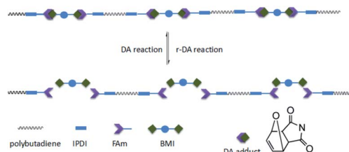
Scheme 2 Thermoreversible self-healing process of FTPB-DA.
