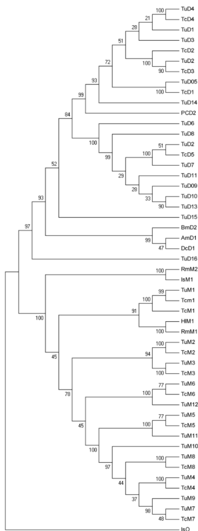
Figure 1. Neighbor-joining phylogenetic analysis of TcGSTs. Reference sequences were obtained from the NCBI database and the genome database of Tetranychus urticae . Pc: Panonychus citri (AFD36890, AFD36888). Tu: Tetranychus urticae (tetur01g02230, tetur01g02470, tetur01g02480, tetur01g02500, tetur01g02510, tetur03g07920, tetur26g01460, tetur26g02801, tetur26g02802, tetur26g01490, tetur26g01500, tetur26g01510, tetur29g00220, tetur31g01330, tetur31g01390, tetur03g09230, tetur05g05180, tetur05g05190, tetur05g05200, tetur05g05210, tetur05g05220, tetur05g05240, tetur05g05250, tetur05g05260, tetur05g05270, tetur05g05290, tetur05g05300). Hl: Haemaphysalis longicornis (AAQ74441). Bm: Bombyx mori (NP_001036974). Am: Apis mellifera (NP_001171499). Dc: Drosophila conformis (AGY31901). Rm: Rhipicephalus microplus (AAD15991, AHH29555, AAL99403). Is: Ixodes scapularis (EEC09568, EEC09568, EEC09120).
