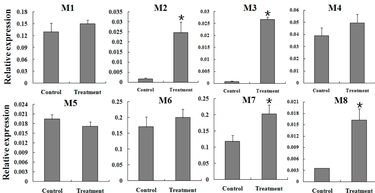
Figure 8. Expression reaction of TcGSTM2 , TcGSTM3 , and TcGSTM8 in female adults of SS to fenpropathrin stimulation.
