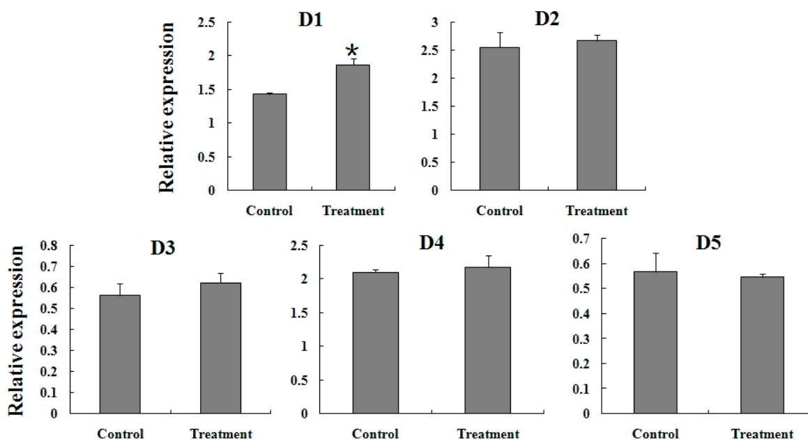
Figure 6. Expression reaction of five delta-class (D1–D5) TcGSTs in female adults of FR to fenpropathrin stimulation. Star above each bar indicate statistical difference determined by t Test ( p < 0.05 ).
