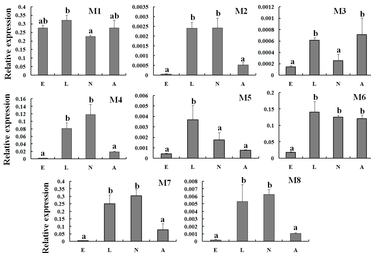
Figure 3. Relative expression of eight mu-class (M1–M8) TcGSTs in different developmental stages. Different letters above each bar indicate statistical difference determined by ANOVA analysis and the Duncan’s Multiple Range Test ( p < 0.05 ). E: Eggs; L: Larvae; N: Nymphs; A: Adults.
