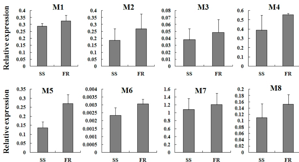
Figure 5. Relative expression of eight mu-class (M1–M8) TcGSTs in female adults of SS and FR. SS: Susceptible strain; and FR: Fenpropathrin-resistant strain.
