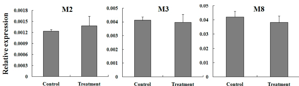
Figure 8. Expression reaction of TcGSTM2 , TcGSTM3 , and TcGSTM8 in female adults of SS to fenpropathrin stimulation.
