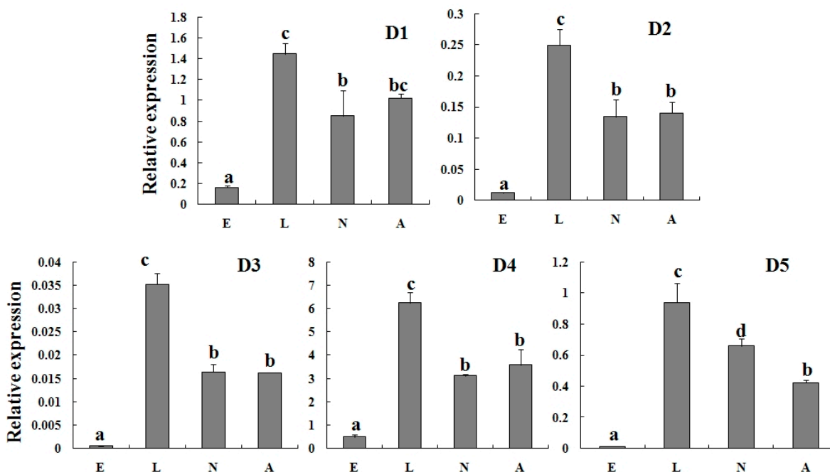
Figure 2. Relative expression of five delta-class (D1–D5) TcGSTs in different developmental stages. Different letters above each bar indicate statistical difference determined by ANOVA analysis and the Duncan’s Multiple Range Test ( p < 0.05 ). E: Eggs; L: Larvae; N: Nymphs; A: Adults.
