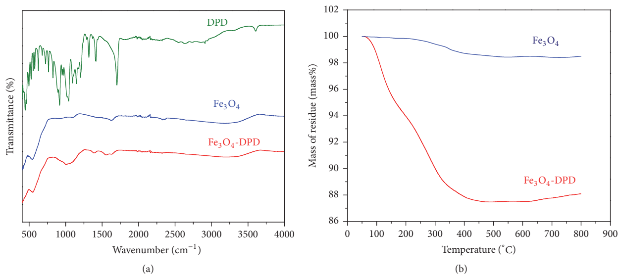
FIGURE 4: (a) ATR-FTIR spectra of DPD, Fe 3 O 4 , and Fe 3 O 4 -DPD MNPs; (b) TGA curves of Fe 3 O 4 and Fe 3 O 4 -DPD MNPs.
