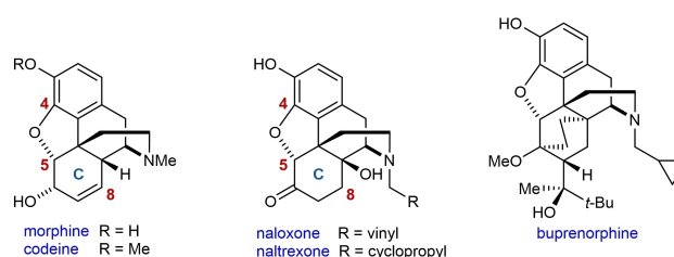
Figure 1. Representative morphinan opioids.
