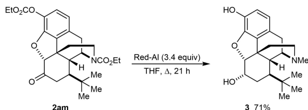
Scheme 2. Removal of the ethoxycarbonyl groups in 2am .
