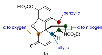
Figure 2. C–H bonds in morphinan opioid 1a with potential HAT reactivity.
