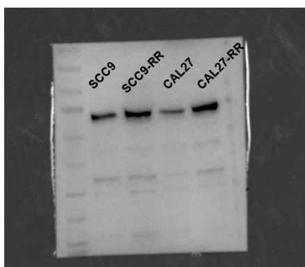
METTL3
