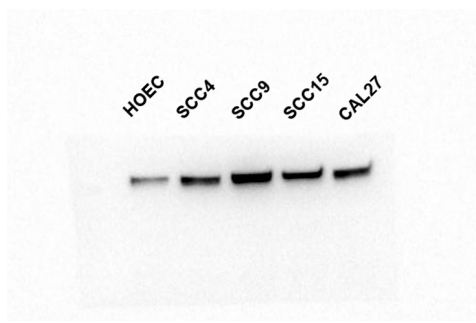
METTL3
