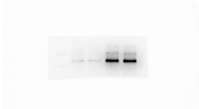
GAPDH
