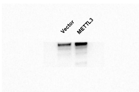
OE-METTL3
