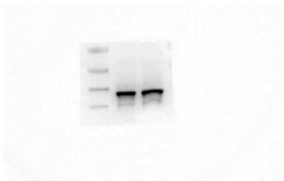
OE-SALL4-GAPDH
