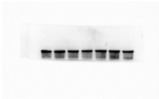
siNC-GAPDH
