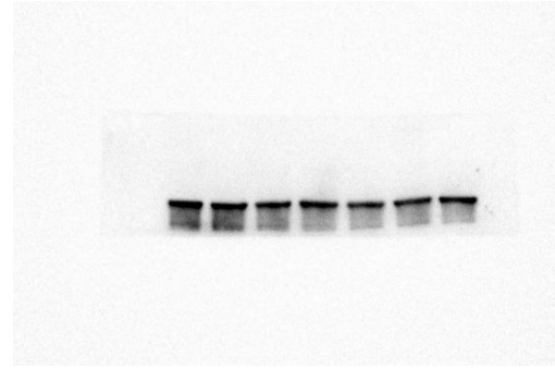
siSALL4#2-GAPDH
