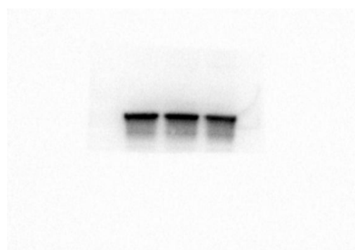
siMETTL3-GAPDH
