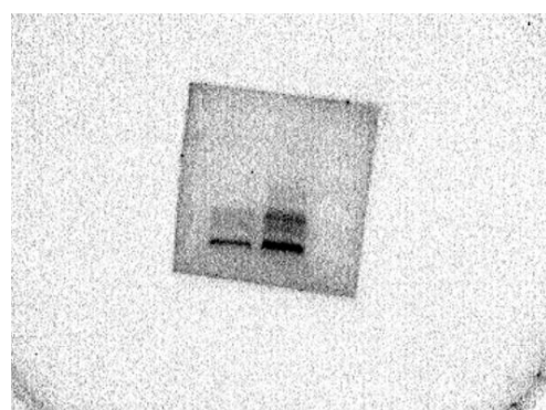
OE-METTL3-OCT4
