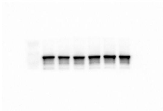
Vector-GAPDH
