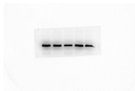
GAPDH
