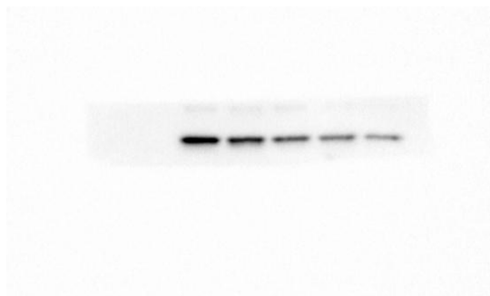
SALL4-H2AX
