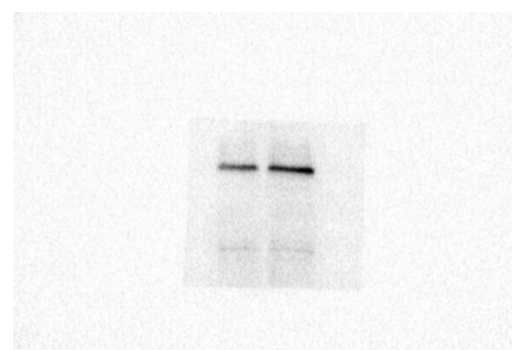
OE-METTL3-SOX2
