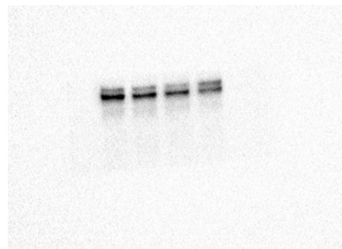
siSALL4-cMYC
