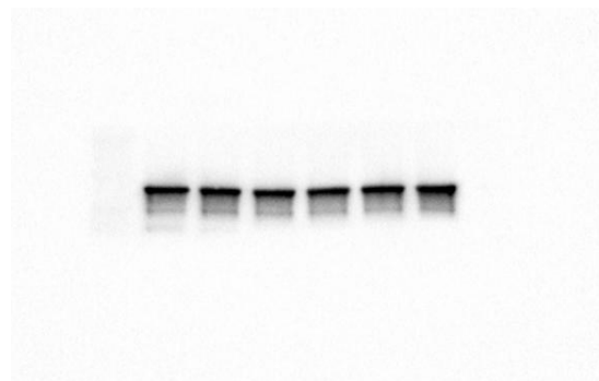
SALL4-GAPDH
