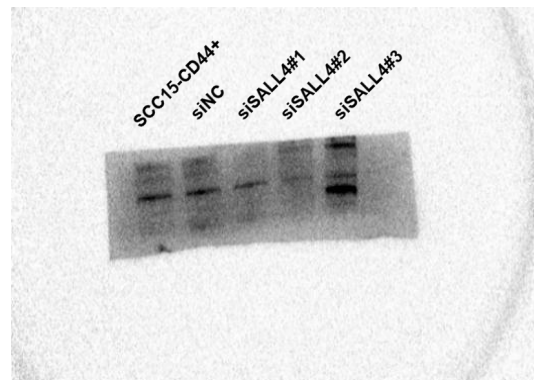
siSALL4
