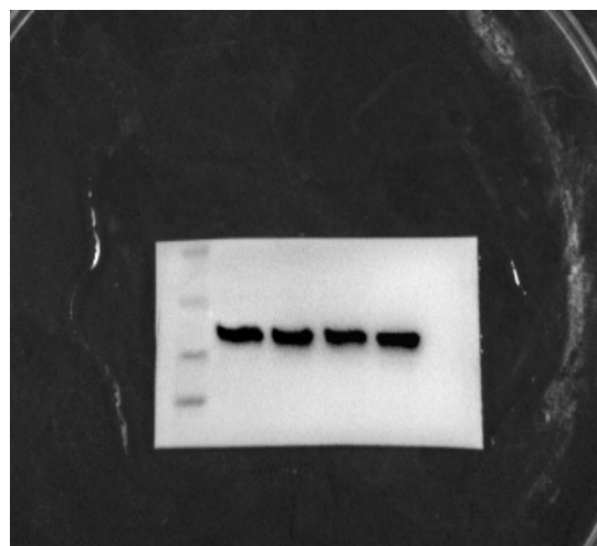
GAPDH
