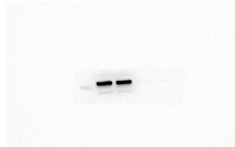
LaminB
