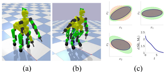
Fig. 17. Tracking of the CoM manipulability with the Centauro robot in simulation. (a) and (b) The initial and final pose of the robot, respectively. (c) Initial, final, and desired manipulability ellipsoids depicted in yellow, dark purple, and green, respectively. The bottom-right graph shows the evolution of the distance between the current and desired manipulability ellipsoid over time (given in seconds).
