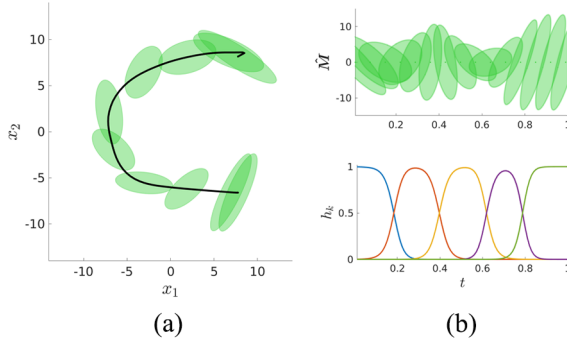
Fig. 4. (a) Desired execution of a C-shape tracking task. The desired Cartesian trajectory and manipulability profile are depicted as a black curve and green ellipsoids. (b) The top shows the desired manipulability ellipsoids estimated by GMR and the bottom shows the influence of GMM components on the time-driven GMR. The colors match the distributions shown in Figure 3(b).
