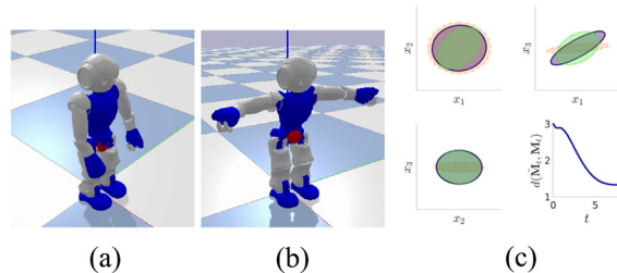
Fig. 18. CoM manipulability tracking with NAO in simulation. (a) and (b) The initial and final pose of NAO, respectively. The CoM of the robot is depicted by a red sphere. (c) Initial, final, and desired manipulability ellipsoids depicted in yellow, dark purple, and green, respectively. The bottom-right graph shows the distance between the current and desired manipulability over time (given in seconds).
