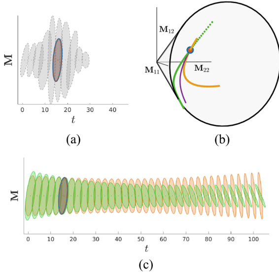
Fig. 10. Importance of geometry in manipulability learning formulations. (a) Demonstrated data (depicted in light gray), and mean of the GMM component for the geometry-aware and Euclidean approaches (overlapping blue and red ellipsoids, respectively). (b) Mean of the GMM component and estimated profiles in the cone of SPD matrices. The manipulability profile obtained by our approach, shown in green, follows a geodesic. The profile obtained by the Euclidean framework is depicted by the orange curve and does not follow a geodesic on the manifold. The geodesic containing the mean of the Euclidean GMM, being a geometrically valid trajectory (depicted in purple), does not correspond to the trajectory obtained with the Euclidean framework. Thus, the Euclidean approach is geometrically flawed. (c) Manipulability profiles retrieved by the geometry-aware and Euclidean GMR, shown as green and orange ellipses, respectively. The time axis is shared with (a).
