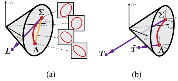
Fig. 2. SPD manifold \mathcal{S}_{++}^2 embedded in its tangent space \text{Sym}^2 . One point corresponds to a matrix \begin{pmatrix} T_{11} & T_{12} \\ T_{12} & T_{22} \end{pmatrix} \in \text{Sym}^2 . Points inside the cone, such as \Sigma and \Lambda , belong to \mathcal{S}_{++}^2 . In (a) L lies on the tangent space of \Sigma such that L = \text{Log}_{\Sigma}(\Lambda) . The shortest path between \Sigma and \Lambda is the geodesic represented as a red curve, which differs from the Euclidean path depicted in yellow. In (b) \tilde{T} \in \mathcal{T}_{\Lambda}\mathcal{M} is the result of the parallel transport of T \in \mathcal{T}_{\Sigma}\mathcal{M} from \mathcal{T}_{\Sigma}\mathcal{M} to \mathcal{T}_{\Lambda}\mathcal{M} . The coordinate axes of the tangent spaces \mathcal{T}_{\Sigma}\mathcal{M} and \mathcal{T}_{\Lambda}\mathcal{M} are represented in dark gray.
