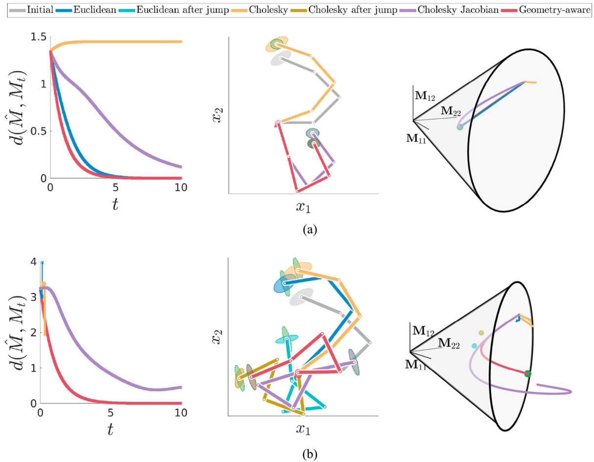
Fig. 11. Performance of different manipulability tracking formulations. The graphs on the left show the affine-invariant distance between the current and desired manipulability ellipsoids over time. The distances for the Euclidean, Cholesky-based Euclidean, Cholesky–Jacobian-based Euclidean and geometry-aware approaches are depicted in blue, yellow, lilac, and red, respectively. The graphs in the middle display the initial and final robot postures and the final manipulability ellipsoids. The initial posture is depicted in light gray, while the final posture and corresponding manipulability for the three methods are depicted in the same color as the distances. The desired manipulability is depicted in green. The middle graph in (b) also shows the sudden change in the robot posture for both Euclidean methods (55) and (56). The robot posture before and after the abrupt change is shown in blue and light blue, respectively, for (55) and in yellow and olive, respectively, for (56). The graphs on the right depict the evolution of the manipulability ellipsoids in the SPD manifold. The colors correspond to those of the previous graphs with the green dot representing the desired manipulability. The isolated light blue and olive dots in the bottom graph in (b) represent the manipulability ellipsoids after the abrupt changes in the robot joint configuration.
