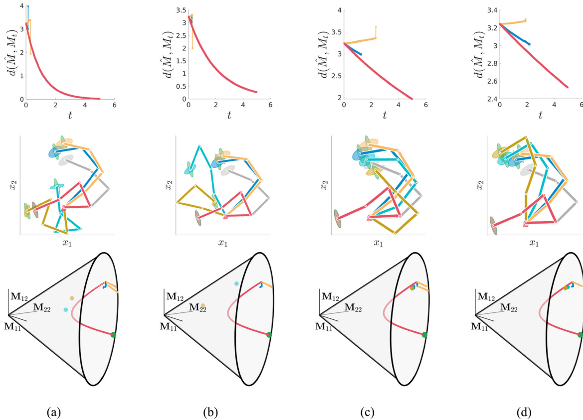
Fig. 12. Comparison of the performance of different manipulability tracking formulations for different gains K_M : (a) K_M = I , (b) K_M = 0.5I , (c) K_M = 0.1I , and (d) K_M = 0.05I . The organization of the graphs and the colors are identical to Figure 11. The Cholesky–Jacobian-based Euclidean formulation is not shown.
