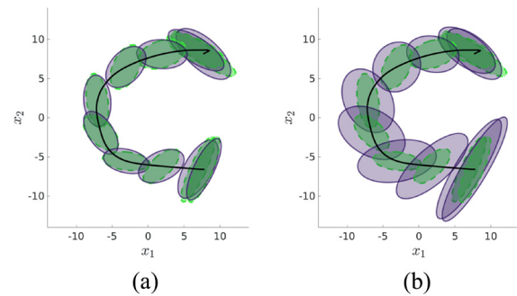
Fig. 8. Reproductions of a learned C-shape tracking task with desired manipulability ellipsoids. The end-effector trajectory is shown in black solid line, while the desired and reproduced manipulabilities are depicted in green and dark purple, respectively: (a) \mathbf{K}_M is a scalar value; (b) \mathbf{K}_M is the diagonal of the precision tensor retrieved by GMR. The required tracking precision is higher at the start and end of the task as a consequence of the low observed variability.
