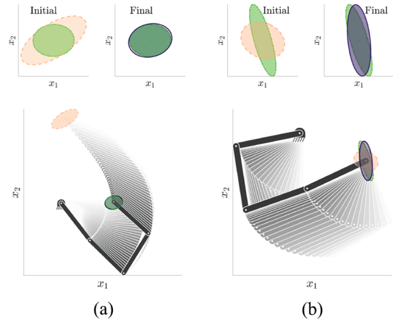
Fig. 5. (a) Manipulability tracking as the main task. (b) Manipulability-based redundancy resolution with Cartesian position control. The robot color goes from light gray to black to show the evolution of the posture. Initial, final, and desired manipulability ellipsoids are depicted in yellow, dark purple, and green, respectively. The top rows show close-up plots corresponding to the initial and final manipulability.
