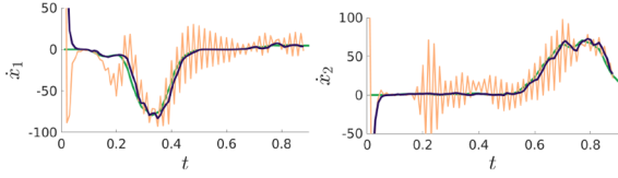
Fig. 15. Cartesian velocities achieved with our manipulability tracking controller (purple) and the volume maximization approach (yellow) as secondary objective for a Cartesian velocity controller. The gain of the velocity controller are equal for both approaches. The desired velocities are shown in green.
