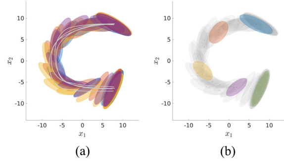
Fig. 3. (a) Four demonstrations of a 3-DoF planar robot tracking a C-shape trajectory. The end-effector path (light gray solid lines) and the manipulability ellipsoids at different time steps are shown for all the demonstrations. (b) Demonstrated manipulability ellipsoids (in gray) and centers \Xi_k of the 5-state GMM in the SPD manifold. Position x and time t are given in centimeters and seconds, respectively.
