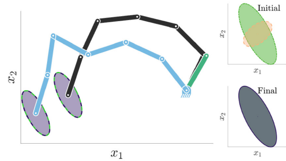
Fig. 9. Use of the nullspace of the manipulability Jacobian. Two 6-DoF planar robots are required to track a desired manipulability ellipsoid as main task. The black robot also keeps its first joint at a fixed position (depicted by the green link), which is a secondary objective projected into the nullspace of the manipulability Jacobian. The final manipulability ellipsoids (in purple) fully overlap the desired ones (in green), showing a precise manipulability tracking. The initial manipulability ellipsoid is depicted in yellow.
