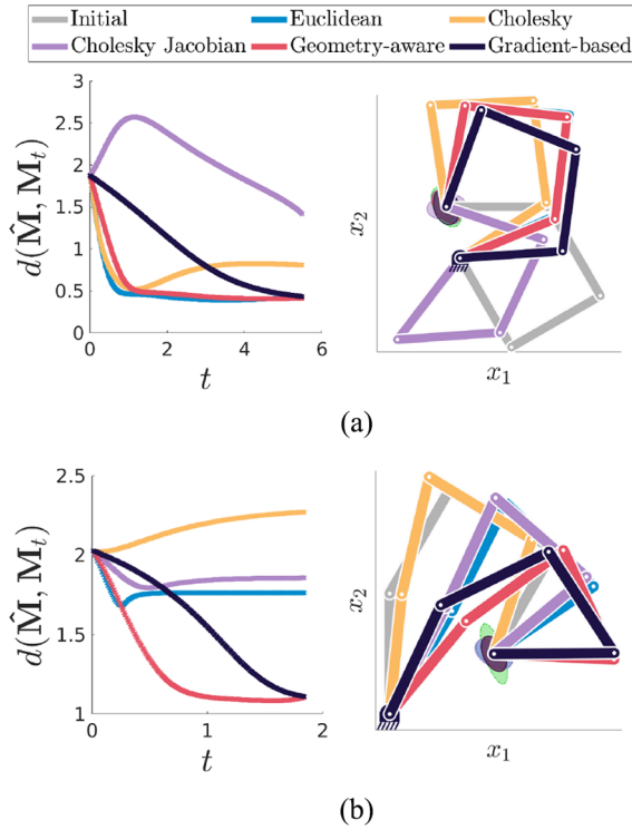
Fig. 13. Performance comparison of the different manipulability-based redundancy resolution formulations. Two cases are shown with varying initial robot configuration and desired manipulability. The graph on the left shows the convergence of the affine invariant distance between the current and the desired manipulability ellipsoid over time. The distances for the Euclidean, Cholesky-based Euclidean, Cholesky–Jacobian-based Euclidean, and geometry-aware and gradient-based approaches are depicted in blue, yellow, lilac, red, and purple, respectively. The graph on the right shows the initial and final posture of the robot along with the final manipulability ellipsoids. The initial posture of the robot is depicted in light gray. The final postures and the corresponding manipulability ellipsoids for the different methods are depicted in the same color as the distances. The desired manipulability ellipsoid is depicted in green.
