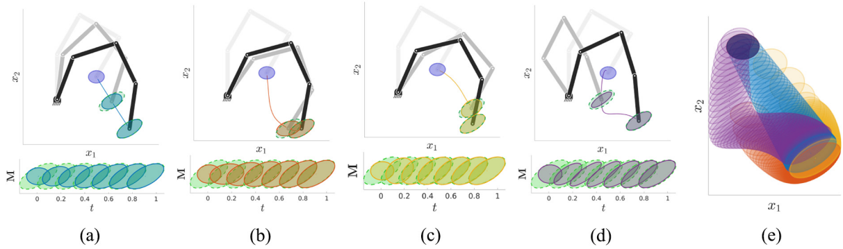
Fig. 7. Manipulability tracking as the main task with diagonal gain matrices defined from different precision tensors. The top plots depict the end-effector trajectory (solid colored line) and the posture of the robot along with the corresponding manipulability at time t = 0, 0.25 , and 1 s. The evolution of the manipulability along time is shown in the bottom plots. (a) Equal tracking precision for all components. (b), (c) Tracking precision is 10:1 higher for x_1 and x_2 , respectively. (d) Correlation between x_1 and x_2 axes is assigned a high tracking accuracy. (e) Evolution of the robot manipulability and end-effector trajectory for the gain matrices used in (a)–(d). The colors match those of the previous graphs. Initial and desired manipulability ellipsoids are depicted in dark blue and green on all graphs. Time t is in seconds.
