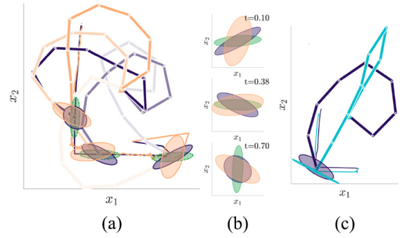
Fig. 14. (a) Comparison of our manipulability tracking controller (in purple) with the manipulability volume maximization (in yellow). The main axis of the desired manipulability ellipsoids (in green) are aligned with the direction of motion in order to allow high velocities during the task execution. The robot colors become darker with the evolution of the movement. (b) Close-up plots of the manipulabilities represented in (a). (c) Comparison of our manipulability tracking controller (in purple) with the compatibility index maximization (in light blue).
