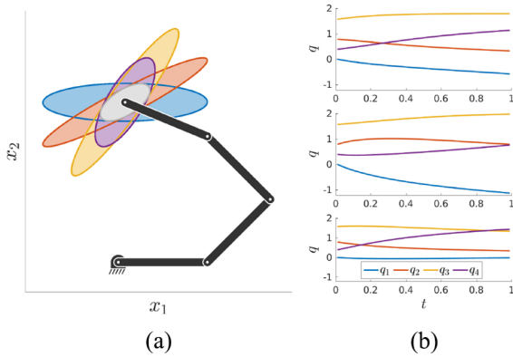
Fig. 6. Illustration of the contribution of actuators. (a) Velocity manipulability ellipsoids obtained when setting a maximum joint velocity, for each joint, five times higher than the rest. The manipulability corresponding to equal maximum joint velocity is shown in gray. (b) Joint trajectories obtained with manipulability tracking (as in Figure 5(a)) for equal maximum joint velocities (top), highest velocity limit for q_1 (middle), and lowest velocity limit for q_1 (bottom).
