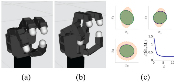
Fig. 16. Manipulability tracking for grasping tasks with the Allegro hand in simulation. (a) and (b) The initial and final pose of the robot, respectively. (c) Initial, final, and desired manipulability ellipsoids depicted in yellow, dark purple, and green, respectively. The bottom-right graph shows the evolution of the distance between the current and desired manipulability ellipsoid over time (given in seconds).
