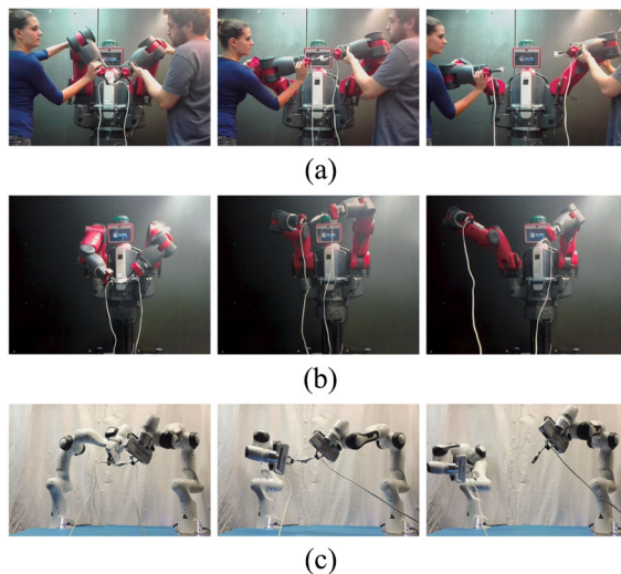
Fig. 19. Unplugging task: (a) demonstrations provided by the user on the Baxter robot; (b) reproduction by the Baxter robot; (c) reproduction by the two Franka Emika Panda robots. The robots pose at the beginning of the task, before, and after the extraction of the cable from the socket are shown in the left, middle, and right column, respectively.
