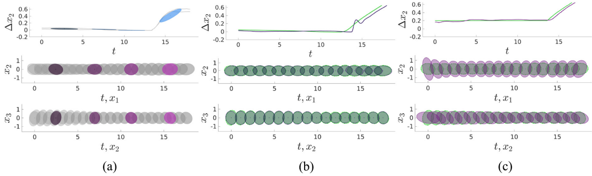
Fig. 20. (a) Demonstrations and GMM encoding the unplugging task. The top graph shows the demonstrated relative end-effectors position for the Baxter robot (in gray) and components of the 4-state GMM (in blue). Only the most representative dimension is displayed. The distance between the two arms increases when the cable is unplugged from the socket. The middle-bottom graphs show the demonstrated force manipulability profile (in gray) and centers of the 4-state GMM in the SPD manifold over time (in purple). (b) Reproduction of the unplugging task with Baxter. The desired and reproduced trajectories are represented in green and dark blue, respectively. The top graph shows the desired and reproduced relative position between the end-effectors along the second dimension. The middle-bottom graphs show the desired and reproduced (overlapping) manipulability ellipsoids. (c) Reproduction of the unplugging task with the two Panda robots. The desired and reproduced trajectories are represented in green and purple, respectively. The top graph shows the desired and reproduced relative position between the end-effectors along the second dimension. The middle-bottom graphs shows the desired and reproduced manipulability ellipsoids. The position x and time t are given in meters and seconds.
