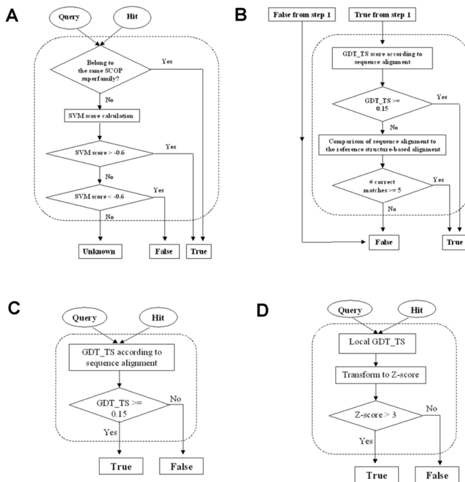
Figure 3 Flowcharts of evaluation of similarity detection. A. Reference-dependent, with no consideration of alignment quality. B. Reference-dependent, with the requirement of alignment quality for true positive hits. C. Reference-independent, global mode. D. Reference-independent, local mode.
