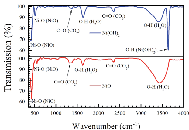
Fig. 3 Fourier-transform infrared response of the precursor Ni(OH) 2 and annealed NiO nanoparticles shows that the oxidation from hydroxide to oxide is complete by annealing at 400 °C for 2 h.
