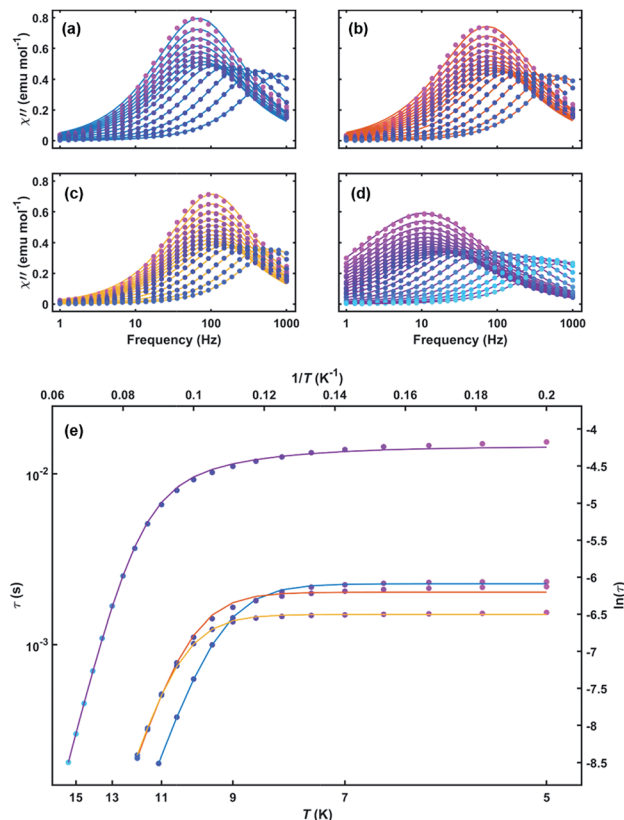
Fig. 3 Out-of-phase susceptibility versus frequency for (a) 1 , (b) 2 , (c) 3 and (d) 4 with both measured data (circles) and Debye model fits (lines). (e) Arrhenius plot of relaxation time versus temperature for 1–4 . Solid lines are fits to eqn (1) ( 1–3 ) and eqn (2) ( 4 ) over all measured temperatures. Line colors: 1 (blue), 2 (red), 3 (orange), and 4 (purple).
