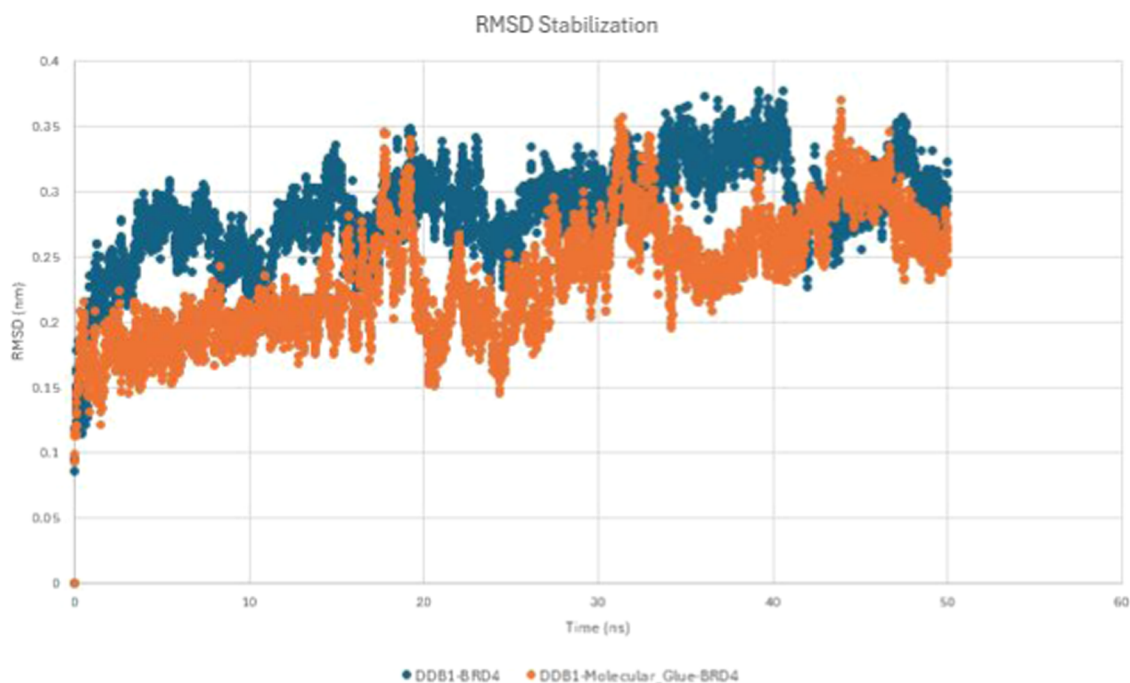
Figure 11. RMSD stabilization of the PDB 8G46 system with and without the molecular glue.
