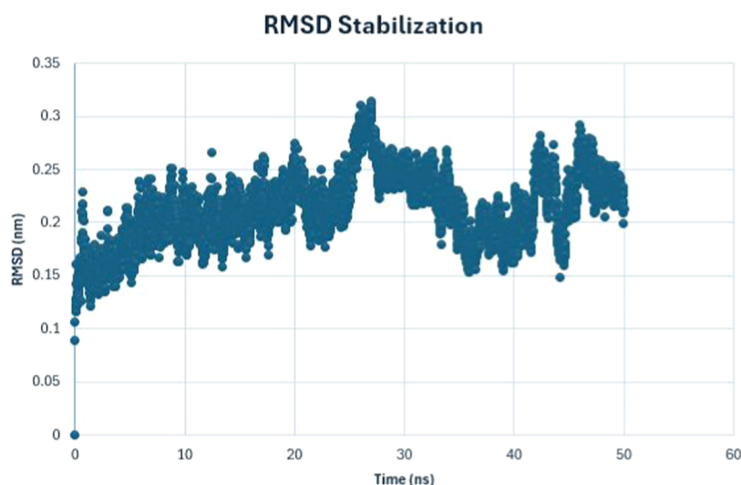
Figure 17. RMSD stabilization of DDB1-Cyclin_dependent_kinase_12 ternary complex stabilized by SAIT_MG_26121.
