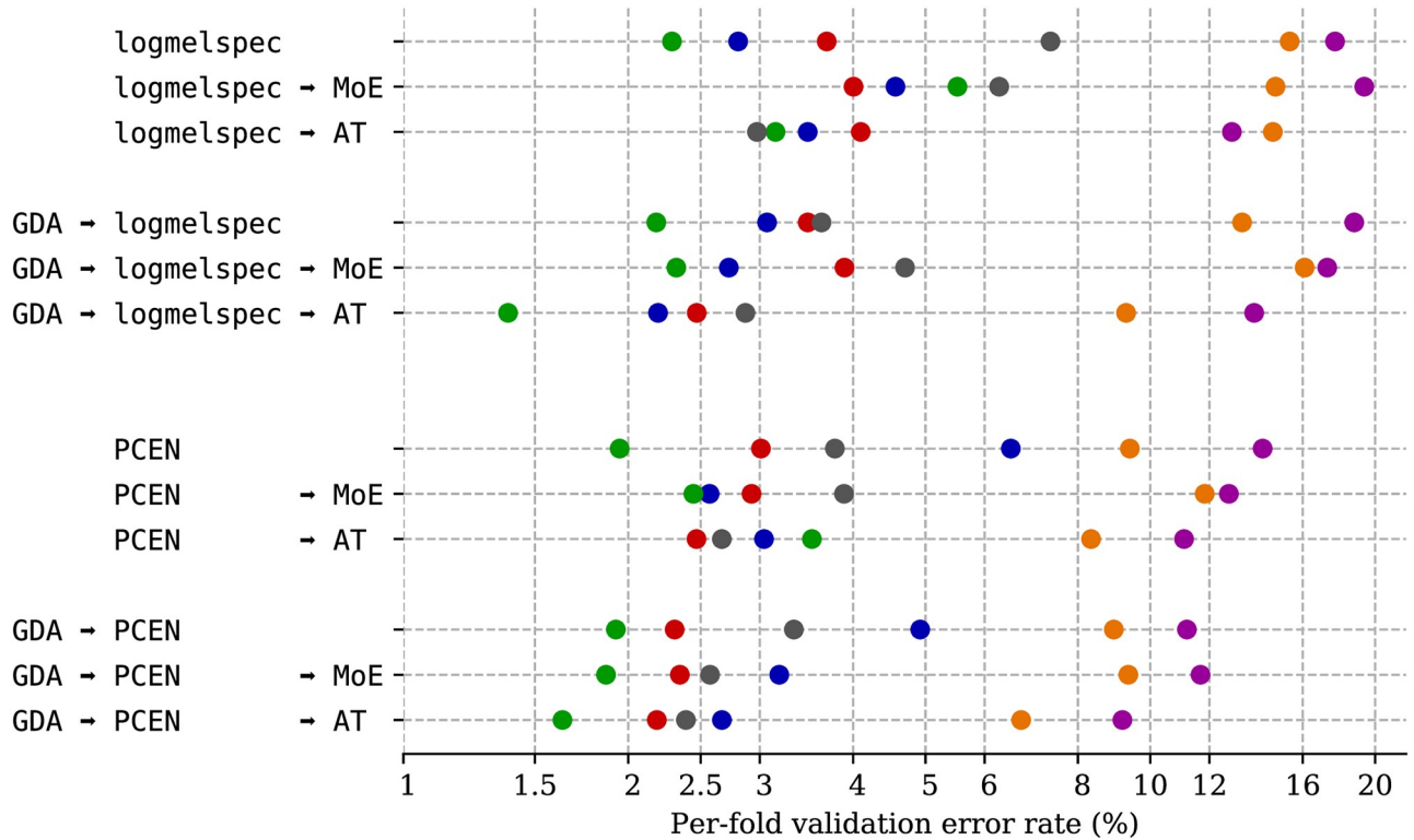
Fig 5. Exhaustive benchmark of architectural variations with respect to the logmelspec-CNN baseline, on a task of binary classification of presence vs. absence of a bird in audio clips. Dot colors represent folds in BirdVox-70k. GDA: geometrical data augmentation. logmelspec: log-mel-spectrogram. PCEN: per-channel energy normalization. MoE: mixture of experts. AT: adaptive threshold.
