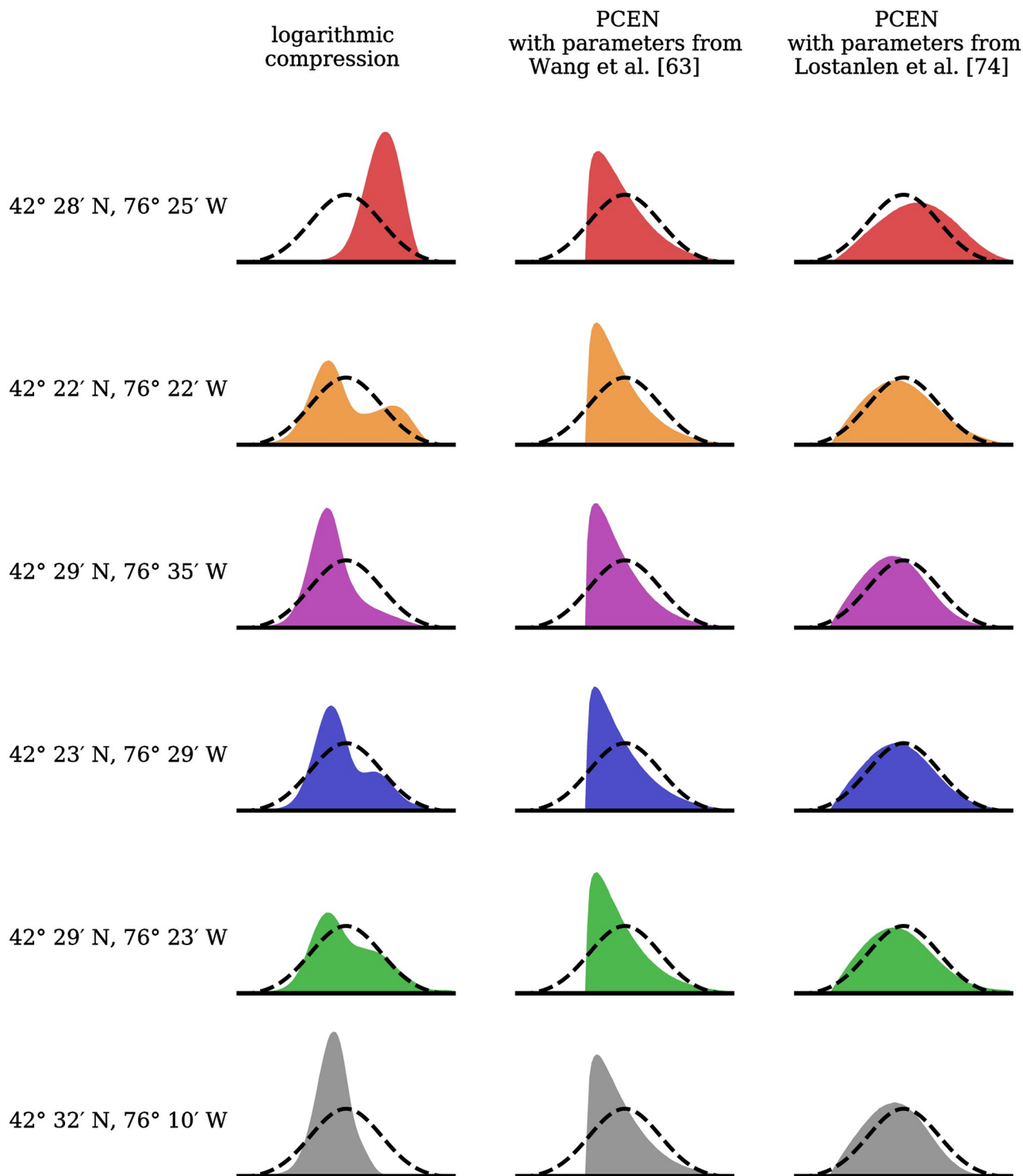
Fig 4. Histogram of magnitudes of time–frequency bins for six one-minute recordings in the BirdVox-full-night dataset, corresponding to six different bioacoustic sensors, for different choices of loudness mapping. Left: after logarithmic compression. Middle: after per-channel energy normalization (PCEN) with the parameters of [63], best suited to automatic speech recognition in a noisy indoor environment. Right: after PCEN with the parameters of [74], best suited to sound event detection in a noisy outdoor environment. We globally standardize the magnitudes in each column to null mean and unit variance. The black dashed line represents the ideal case of a standard normal distribution. The text on the left of each row denotes the latitude and longitude of the corresponding autonomous recording unit in the acoustic sensor network. See text for details about parameter settings.
