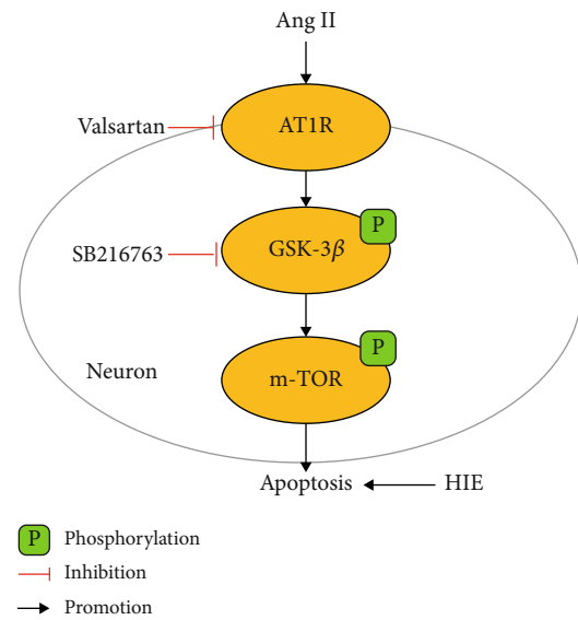
FIGURE 1: Graphic illustration for Ang II mediated neuronal apoptosis in Hypoxic-ischemic encephalopathy.
