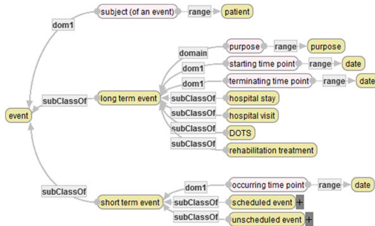
Figure 10 Basis concepts and attributes related to events (partial).
