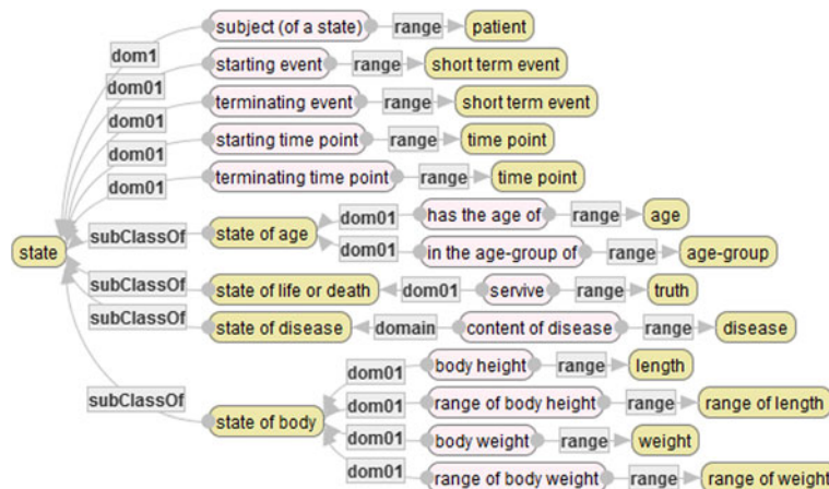
Figure 11 Basis concepts and attributes related to states of patients.
