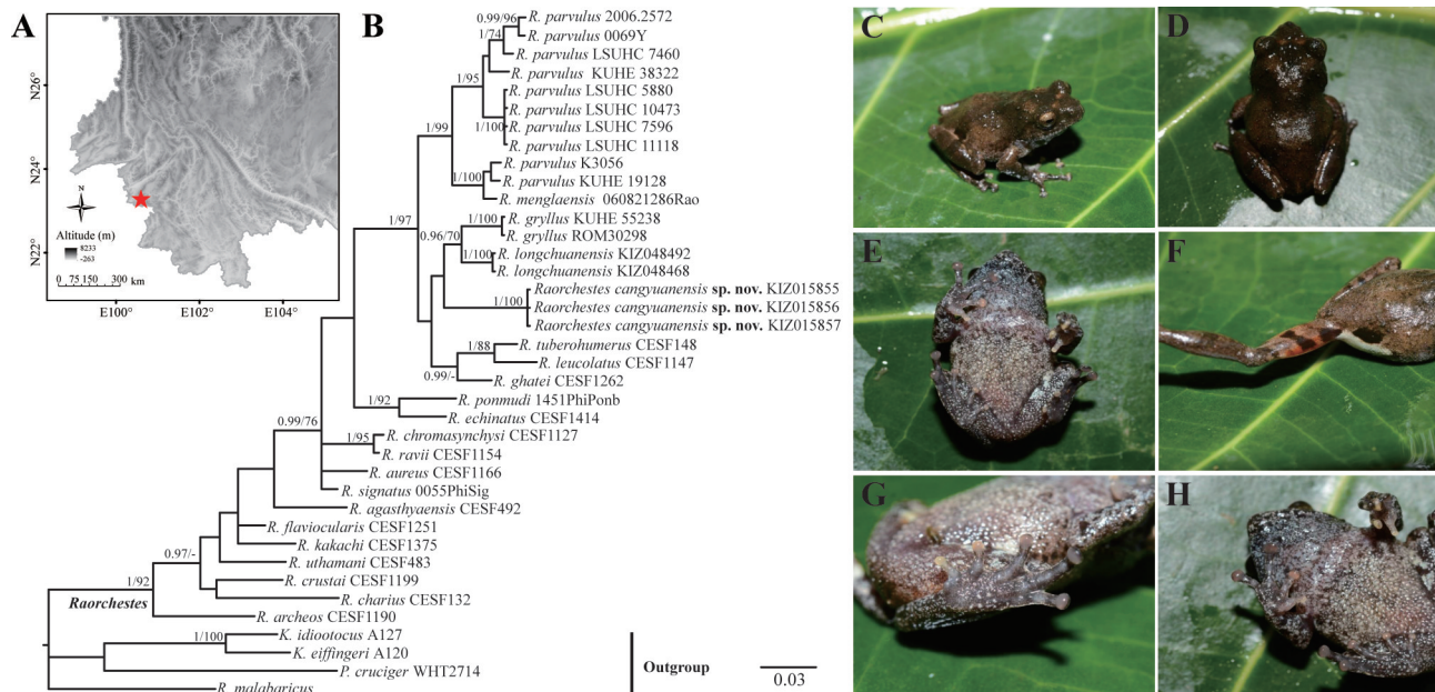
Figure 1 Distribution, Bayesian inference tree and holotype of Raorchestes cangyuanensis sp. nov.
