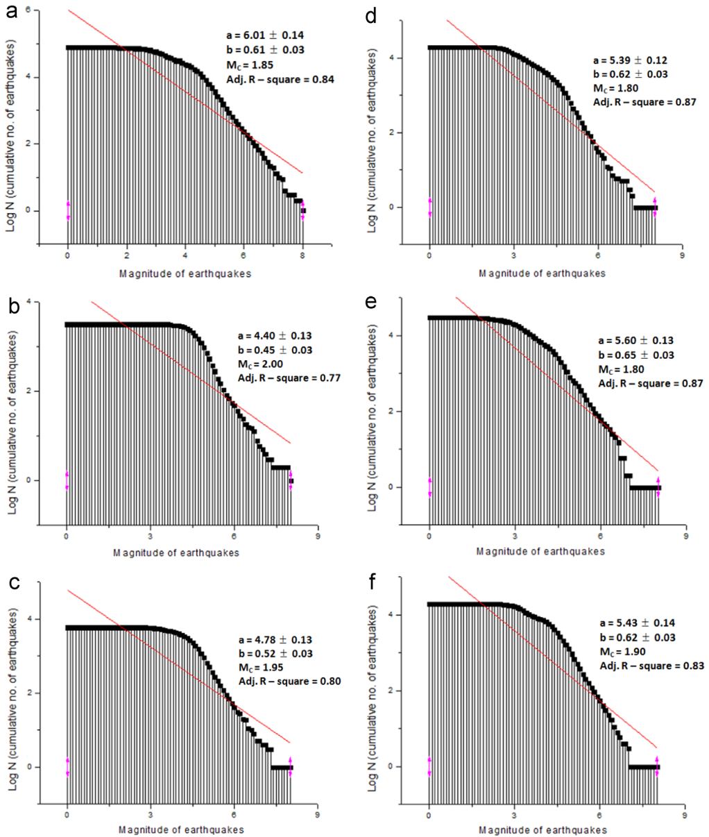
Fig. 7. a. Log N – magnitude distribution from 1966 to 2015 b. Log N – magnitude distribution from 1976 to 1985 d. Log N – magnitude distribution from 1986 to 1995 e. Log N – magnitude distribution from 1996 to 2005 f. Log N – magnitude distribution from 2006 to 2015.
