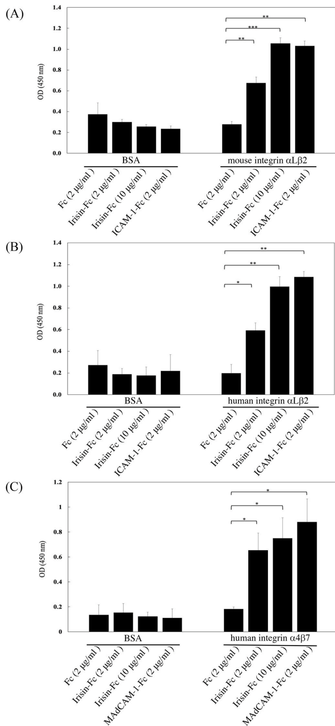
Fig. 5. Purified protein based-ELISA type experiments to study the interaction of irisin with integrin αLβ2 and α4β7. Binding of irisin- or control-Fc to immobilized proteins such as; mouse αLβ2 (A), human αLβ2 (B), human α4β7 (C), and BSA as a control (A–C); was examined. (A–C) Data are expressed as the mean ± SEM of three independent experiments carried out in triplicate. *p < 0.05, **p < 0.01, ***p < 0.001 compared with control Fc in each group.
