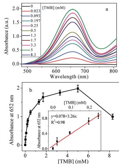
Fig. 4 (a) Absorption spectra of the sensing platform with increasing the concentration of TMB ( \text{H}_2\text{O}_2 : 20 mM). (b) The linear relationship between the relative absorption intensities and the concentration of TMB. Inset is the linear relationship in the low concentration. The error bars represent the standard deviation of three independent measurements.
