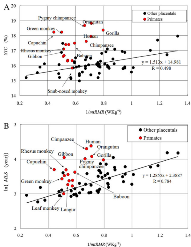
FIG. 3. —(A) Relationship between 1/\text{mtRMR} and STC in placentals. (B) Relationship between 1/\text{mtRMR} and \ln(\text{MLS}) . The placentals of (A) exclude cetaceans, sirenians, rodents, and insectivores.
