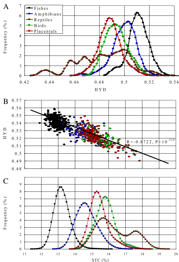
FIG. 1. —(A) Frequency distribution of HYD over vertebrates. (B) Correlation between STC and HYD. (C) Frequency distribution of STC. The correlation became very strong in a hydrophobic domain of MMPs with S_{av} > 0.1 ( R = -0.8722 and P < 10^{-220} ). Here, S_{av} is the moving average of local hydrophobic scores S around each amino acid site (Materials and Methods).
