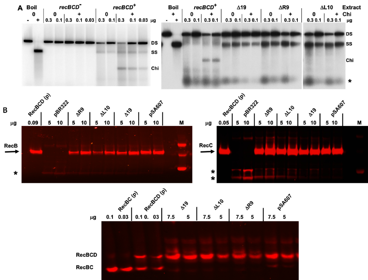
Figure 4. The RecB tether is required for full Chi-cutting activity but not enzyme assembly or DNA unwinding. Extracts were prepared from late log-phase cells of strain V2831 ( \Delta recBCD2731 ) containing derivatives of plasmid pSA607 ( recBC 2773D ) with the indicated recB tether deletion. (A) DNA unwinding and Chi cutting were assayed using HindIII-linearized 32 P-labeled pBR322 \chi^0 or \chi^+ F225 DNA. The indicated amount of extract protein, per 15 \mu l reaction, was reacted with the DNA substrate (0.8 nM) at 37° for 2 min and the products separated on a 0.9% agarose gel. The positions of dsDNA substrate (DS), unwound ssDNA (SS; boiled), the product of Chi-dependent cutting (Chi), and limit-digest oligonucleotides (*) are shown. (B) RecB and RecC polypeptides and native forms of RecBCD enzyme in extracts of RecB tether mutants were separated on 3–8% Tris-acetate native or SDS denaturing polyacrylamide gels and detected by Western blots using the indicated polyclonal antibodies. Purified (p) RecBCD or RecBC enzyme was run as a marker. The lane with size markers (150, 120, and 65 kDa, top to bottom) is indicated (M). The migrations of RecB and RecC polypeptides and of RecBCD heterotrimer and RecBC heterodimer are indicated. Cross-reacting polypeptides present in extracts of V2831 containing pBR322 but lacking RecBCD are indicated (*). See Supplementary Figures S5 and S6 for additional data.
