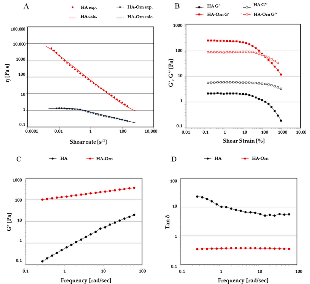
Figure 7. The trend of viscosity values (panel A), G' and G'' moduli (panel B), complex moduli ( G^* ) (panel C), and damping factor ( \tan \delta ) (panel D).
