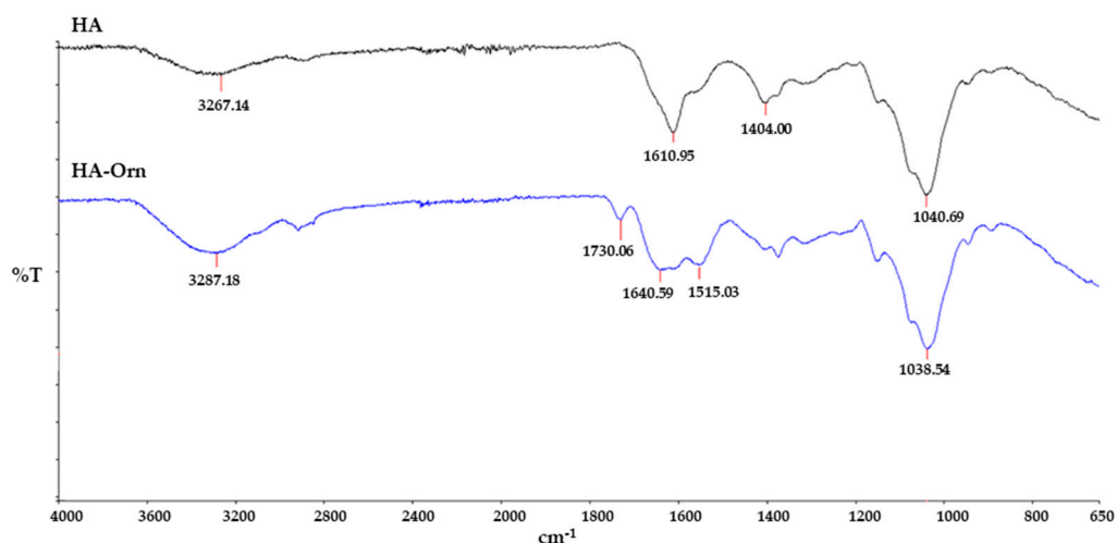
Figure 3. FTIR spectra of native HA and cross-linked HA–Orn.
