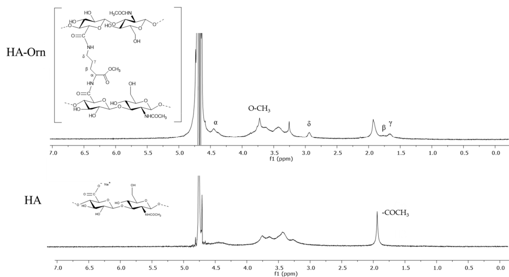
Figure 2. 1 H-NMR spectrum of native HA and cross-linked HA–Orn recorded in D 2 O.
