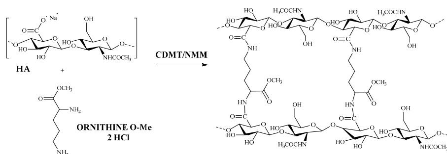
Figure 1. Synthetic scheme of HA crosslinked with the Ornithine methyl ester.
