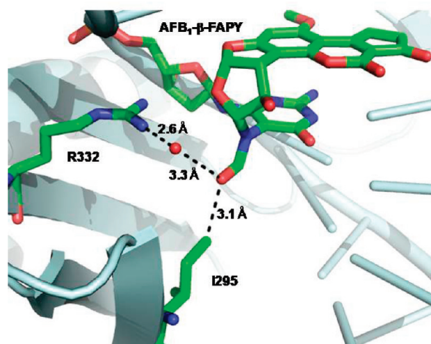
Figure 8. The water-mediated hydrogen bond network for the ternary complex with AFB 1 - \beta -FAPY-modified Sequence II template:primer complex with the S. solfataricus P2 DNA polymerase Dpo4 and incoming dATP. The red sphere represents the oxygen atom of a water molecule. The distances are measured between the donor and acceptor atom.
