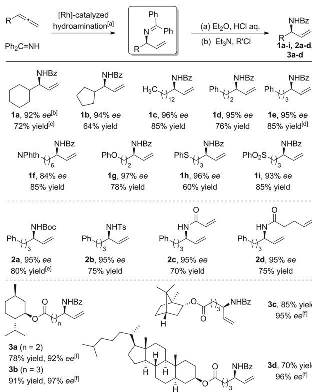
Scheme 3 Scope of allenenes and one-pot synthesis of allylic amides. [a] Benzophenone imine (1.0 equiv., 0.4 mmol), allene (1.5 equiv.), [(Rh(COD)Cl) 2 ] (2.0 mol%), L4 (4.0 mol%), PPTS (20 mol%), DCE (1.0 ml). [b] Determined by chiral HPLC. [c] Yield is that of the isolated product. [d] The reaction was performed in 0.2 mmol scale. [e] Boc 2 O was used in the protection step. Phth = phthaloyl; Ts = 4-methylbenzene-1-sulfonyl. [f] Determined by chiral HPLC after transesterification with ethanol.
