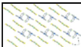
Fig. 3. Packing of [Fbzql][Ni(dmit) 2 ] viewed along c -axis
