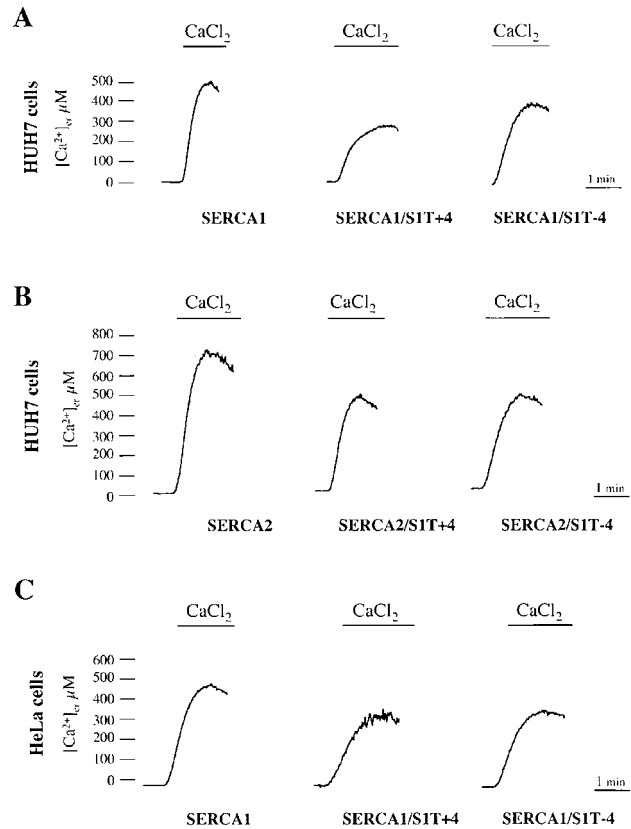
Figure 6. S1T proteins reverse SERCA1- and SERCA2b-induced increases of [Ca^{2+}]_{er} . HuH7 (A and B) and HeLa (C) cells were cotransfected with erAEQ and SERCA1 (A and C) or SERCA2b (B). Cotransfection of erAEQ, SERCA1, or SERCA2b and S1T constructs was carried out as described in Materials and Methods. Quantitative assessment of [Ca^{2+}]_{er} was performed as described in the legend to Fig. 5.
