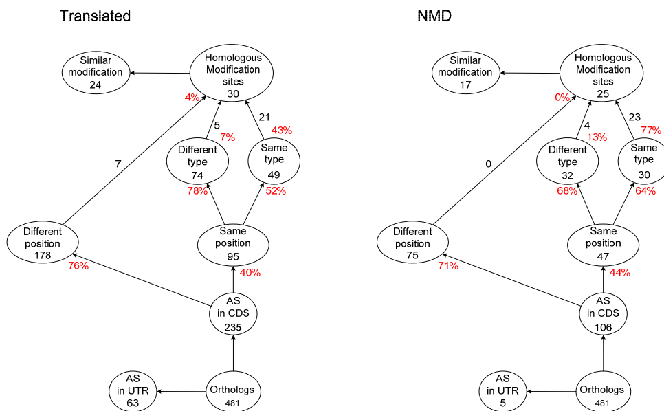
Dissection of AS events in orthologous genes. A schematic view is provided of the dissection of AS events in Arabidopsis-rice orthologs (A) and maize-rice orthologs (B). The dissection is given for both the translated- and NMD set. Number of orthologous genes within each category is indicated below the name of the category. Numbers next to arrows represent the number of pairs within the category from which the arrow originates that contribute to the number of pairs within the category pointed to by the arrow. For a number of classes the fraction of ortholog pairs from its preceding class that is contained within the child class is provided (in red). Note: several ortholog pairs can be represented in more than one child class as a number of genes have more than one AS variant.
