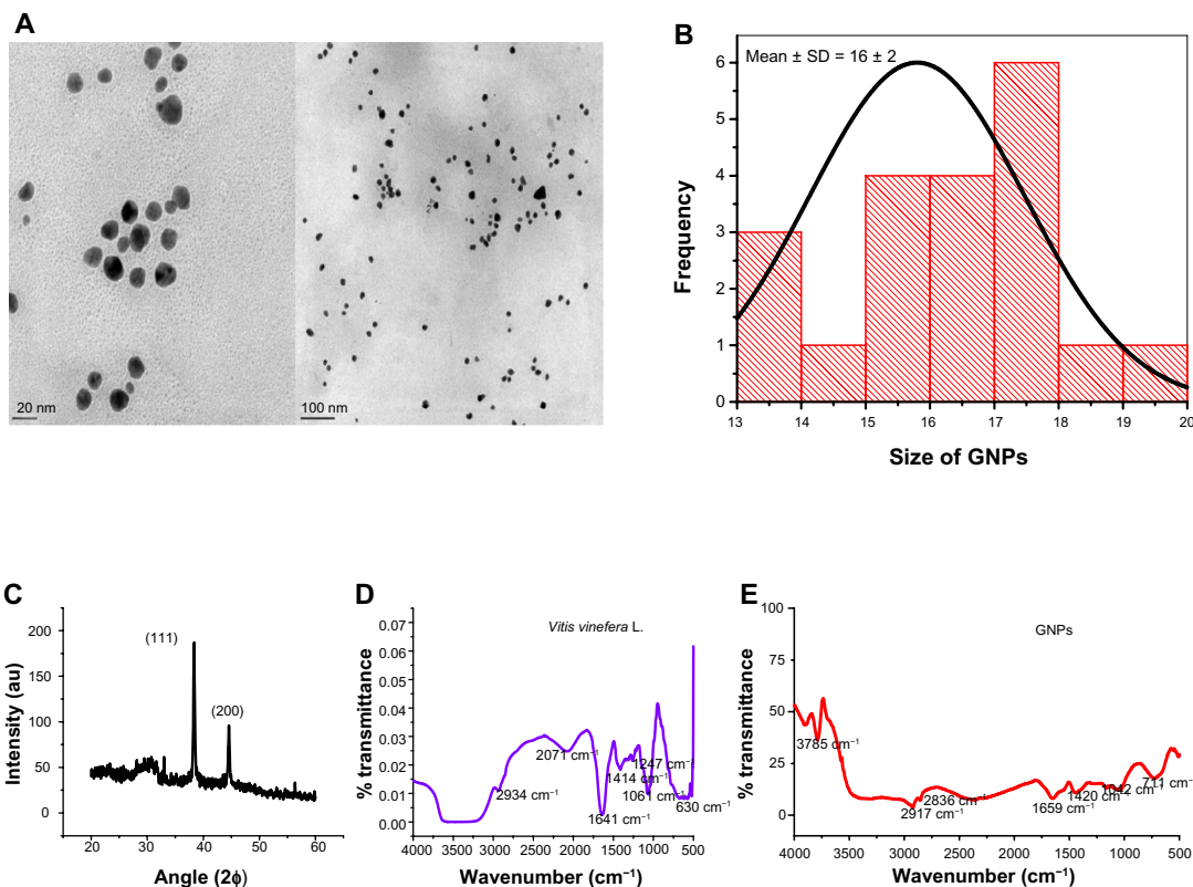
Figure 3 (A–E) Characterization of GNPs (16 ± 2 nm). (A) TEM showing GNP shape and size. The analysis was carried out at an accelerating voltage of 200 kV. The particles were measured on two different scales: 20 nm and 100 nm. (B) Histogram showing average size of GNPs measured by TEM. (C) X-ray diffraction spectra from the particles. The particles were recorded at 40 kV voltage and 40 MV current using Cu-K \alpha radiation ( \lambda = 1.5405 \text{ \AA} , scan rate 1°/minute). (D and E) Fourier-transform infrared spectra of Vitis vinifera L. and GNPs. The spectrum was recorded from 500 to 4,000 \text{cm}^{-1} from the GNPs in the transmittance mode using KBr crystal.
