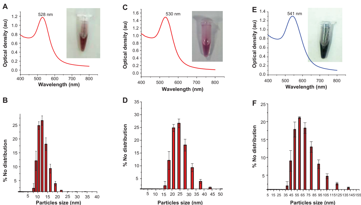
Figure 2 UV-vis spectra of the different sizes of GNPs: (A) 14 nm; (C) 28 nm; (E) 61 nm. Dynamic light-scattering histograms showing particle distribution of GNPs: (B) 14 ± 1 nm; (D) 28 ± 2 nm; (F) 61 ± 2 nm.
