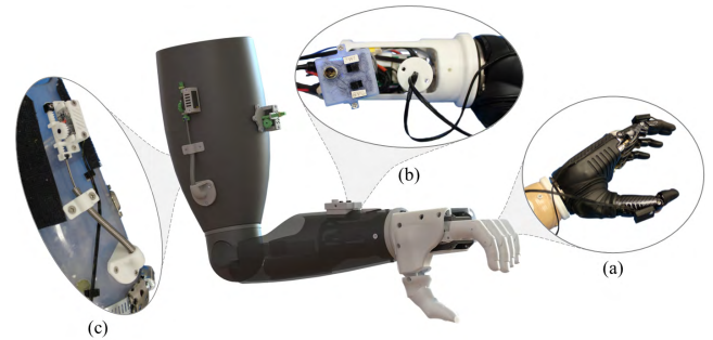
FIGURE 1. Schematic of mechanotactile factor system (a) sensors, (b) electronics, and (c) tactor.
