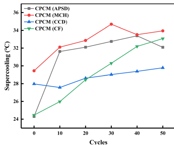
Fig. 12 Cyclic supercooling of CPCMs.
