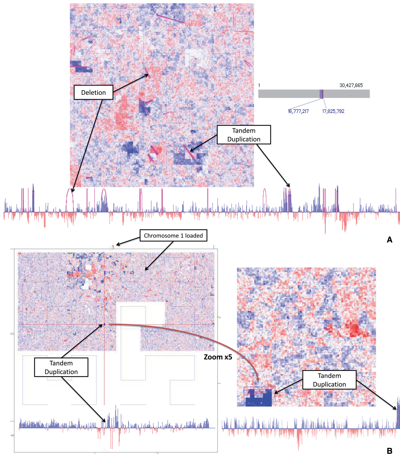
Figure 3. Comparison of chromosome 1 between strain ICE153 from central Asia and strain ICE97 from southern Italy. (A) An example of a deletion and a tandem duplication supported by both pair-end and read-depth information. (B) The advantage of the Hilbert representation. Left: A tandem duplication that is not visible in the linear representation (1 pixel length) but very clear in the Hilbert representation as a bigger block. Right: The same tandem duplication at zoom level 5 supported both by read-depth and pair-end evidence.
