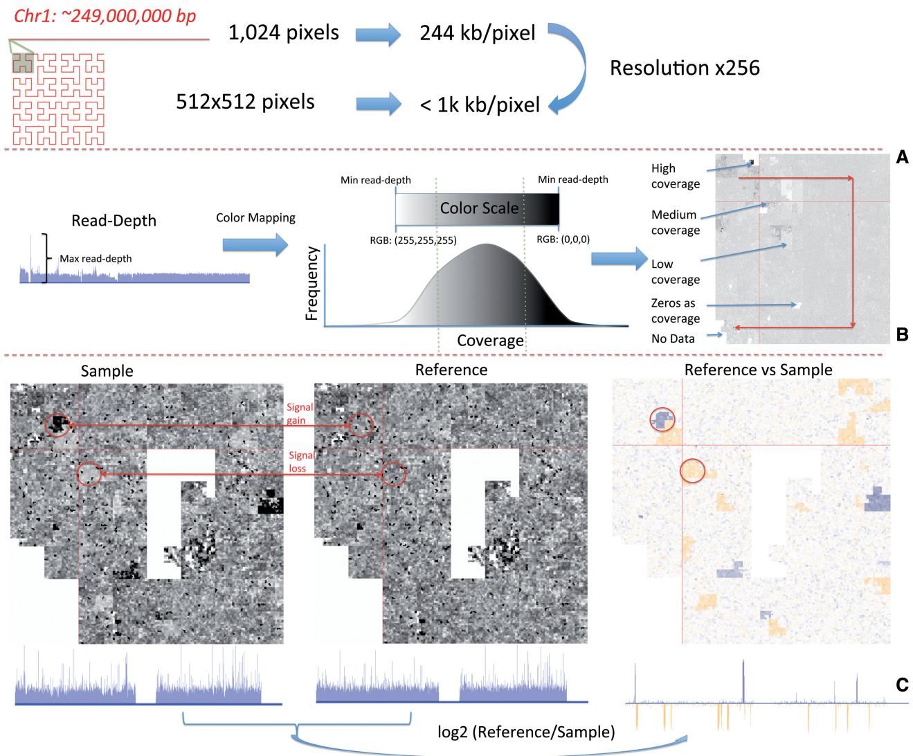
Figure 2. Space filling curves in genomic data. (A) Resolution gain comparing the linear with the Hilbert representation. (B) Colour mapping: The transparency of the colour is adjusted according to the signal value. Dark areas indicate high coverage; light grey areas lower coverage. White areas indicate zero coverage or absence of data. The red arrows show the coordinate system of the system curve. (C) Comparison of a sample against a reference: Left : The sample and reference human chromosome 1 in both a Hilbert and a linear representation. Right : The log 2 ratio between the reference and the signal. Blue signals indicate possible tandem duplications as reference < sample, and yellow blocks indicate possible deletions as reference > sample.
