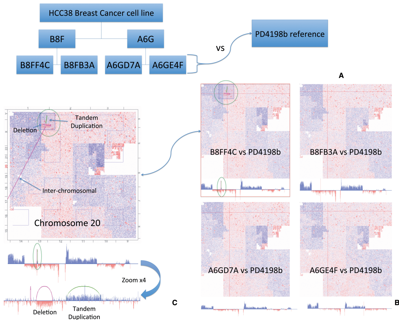
Figure 4. The unstable nature of HCC38. (A) Hierarchy of the single-cell derived subclones and comparison with the PD4198b reference genome. (B) Comparison between the four subclones against the PD4198b reference genome. Subclone B8FF4C demonstrates a de novo tandem duplication and flanking deletion not present in the other subclones. (C) Visualization of an inter-chromosomal variation (linked to the q-arm of chromosome 17), a unique deletion and tandem duplication around position 15200000 for chromosome 20 not present in the other subclones.
