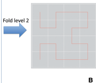
Figure 1. Folding levels of a Hilbert curve. The number of the edges of the Hilbert curve is 4^N , where N denotes the fold level. For a canvas of 2^9 \times 2^9 = 512 \times 512 = 262144 pixel dimension, the fold level N = 9 covers every pixel of the plane.
