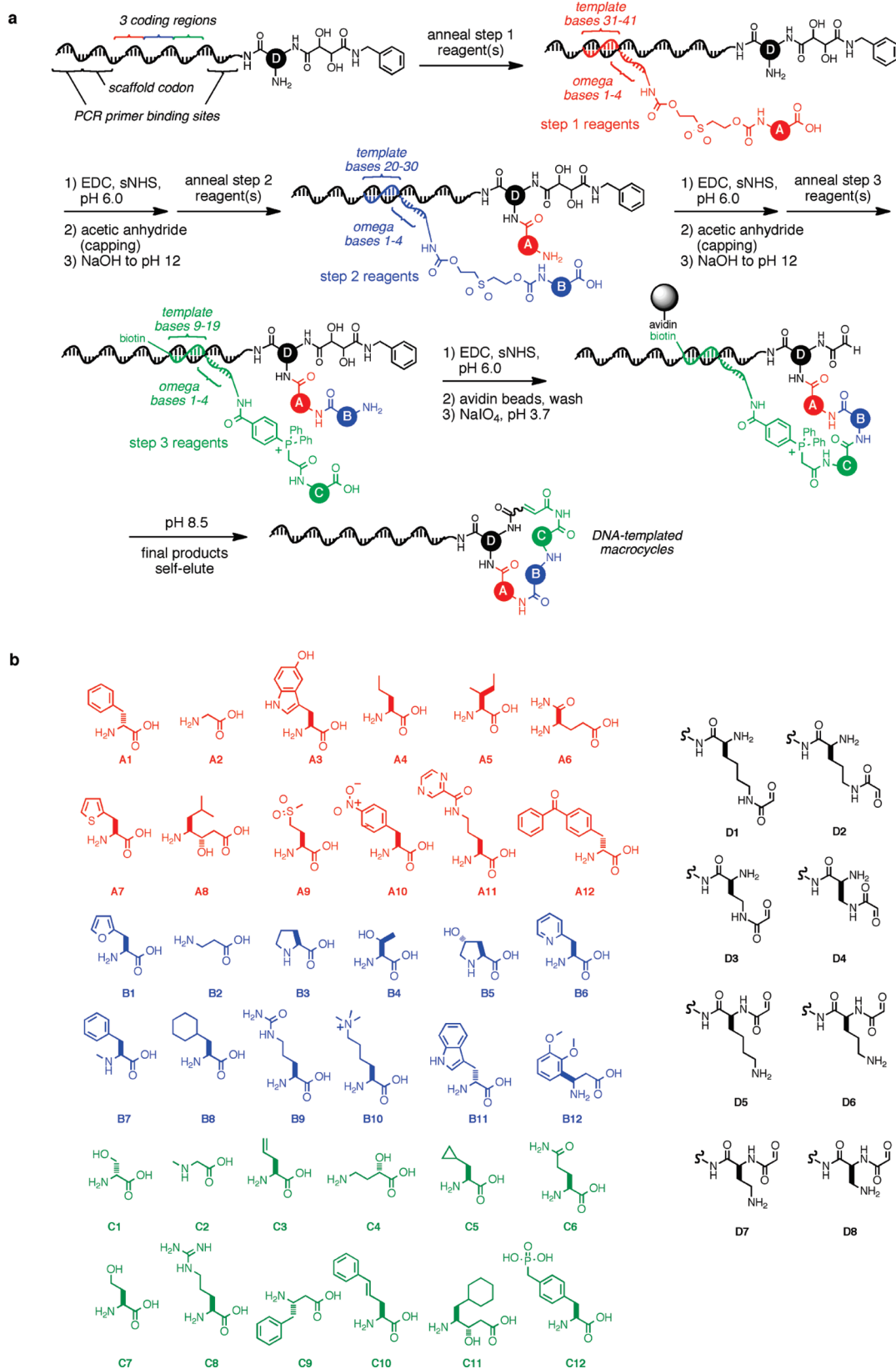
Figure 1. The 13 824-membered DNA-templated small-molecule macrocycle library. (a) Scheme for the multistep DNA-templated synthesis of the macrocycle library. 24 (b) Amino-acid building blocks used in the library synthesis. Step one building blocks (A1–A12) are shown in red, step two building blocks (B1–B12) are shown in blue, step three building blocks (C1–C12) are shown in green, and the macrocycle scaffolds (D1–D8) are shown in black.
