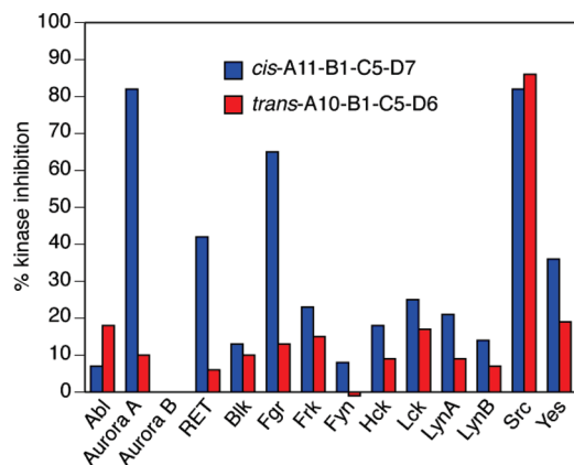
Figure 7. Selectivity of macrocycles cis -A11-B1-C5-D7 and trans -A10-B1-C5-D6 among Src-related kinases, including all nine Src-family kinases. Both macrocycles were assayed at 5 \mu\text{M} concentration against the indicated kinases. Assays of cis -A11-B1-C5-D7 against Abl and Hck were performed at 50 \mu\text{M} macrocycle concentration instead of 5 \mu\text{M} . Percent kinase inhibition values plotted are the average of two independent measurements. Assay data for Src kinase is from Figure S2 and Table 3. All non-Src assay points were measured by the Invitrogen Select Screen Profiling Service.
