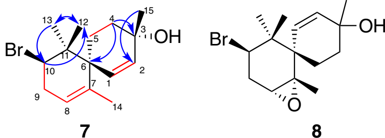
Figure 2 Important HMBC (blue arrows) and COSY (bold bonds) correlations for 7 , and the chemical structure of the related 10-bromo-7,8-epoxychamigr-1-en-3-ol ( 8 ).
