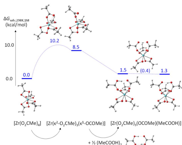
Fig. 8 Gibbs energy profile ( 25 \text{ }^\circ\text{C} in dichloromethane, 1 \text{ M} standard state) of the chelating acetate exchange in [\text{Zr}(\text{O}_2\text{CMe})_4] .
