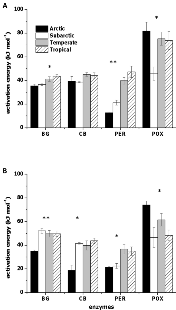
Figure 1. Activation energy for hydrolytic and oxidative enzymes. E_a in (a) A horizon and (b) B horizon for \beta -glucosidase (BG), cellobiohydrolase (CB), peroxidase (PER) and phenol oxidase (POX). Activation energy calculated from three subsamples taken from each soil and depth combination. The number of study locations per biome were tropical n=2 ; temperate n=3 ; subarctic n=1 ; arctic n=1 . The “*” indicates a significant effect of biome with a 0.05 \leq P \leq 0.1 and “**” indicates a significant effect of biome with a P \leq 0.01 . doi:10.1371/journal.pone.0059943.g001
