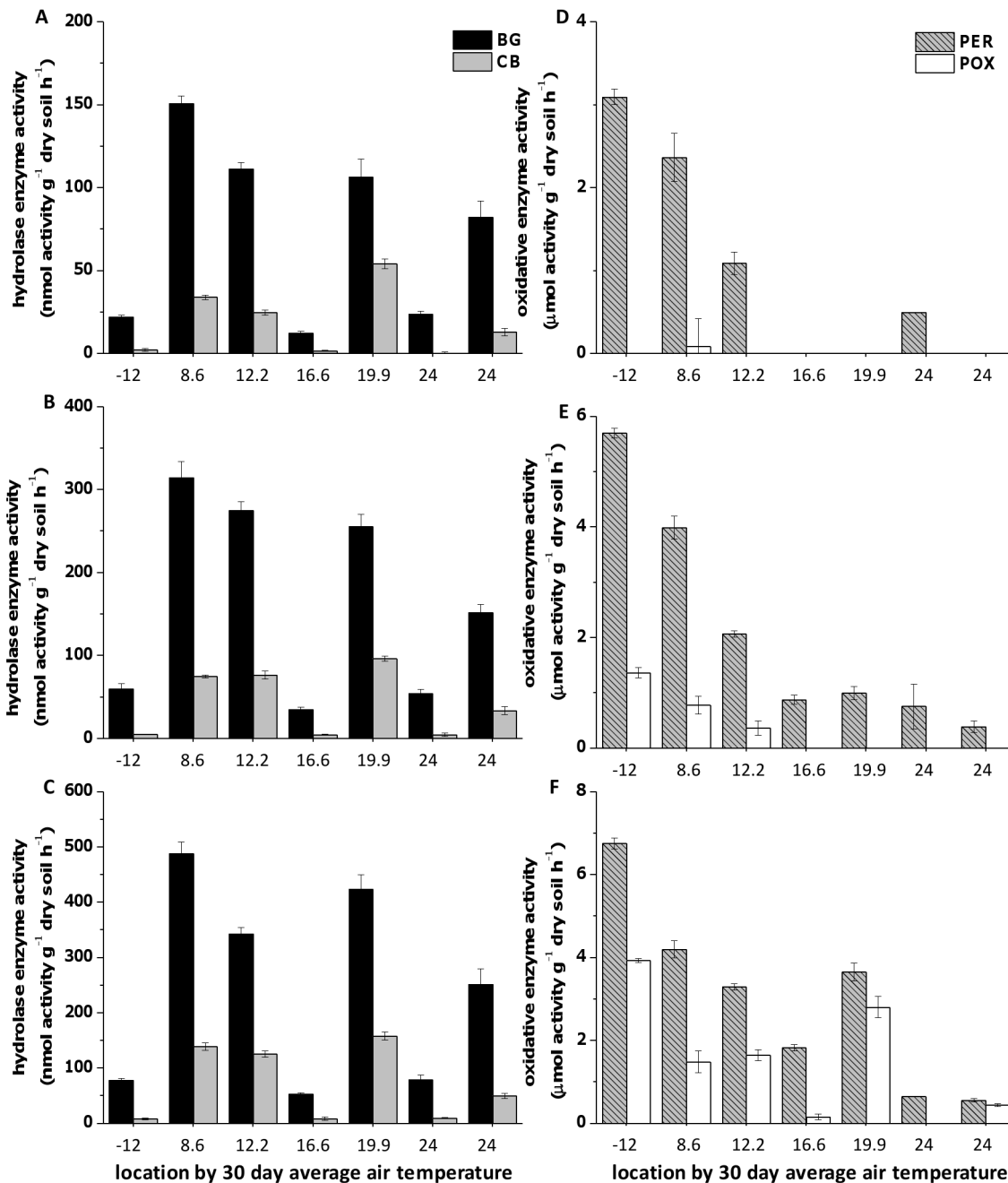
Figure 2. Hydrolytic and oxidative enzyme activities in the A horizon. Enzyme activities at (a) 4°C, (b) 21°C, and (c) 30°C for hydrolytic enzyme activities in order by average air temperature 30 days prior to sampling. Oxidative enzyme activity at (d) 4°C, (e) 21°C, and (f) 30°C in order by average air temperature 30 days prior to sampling. doi:10.1371/journal.pone.0059943.g002
