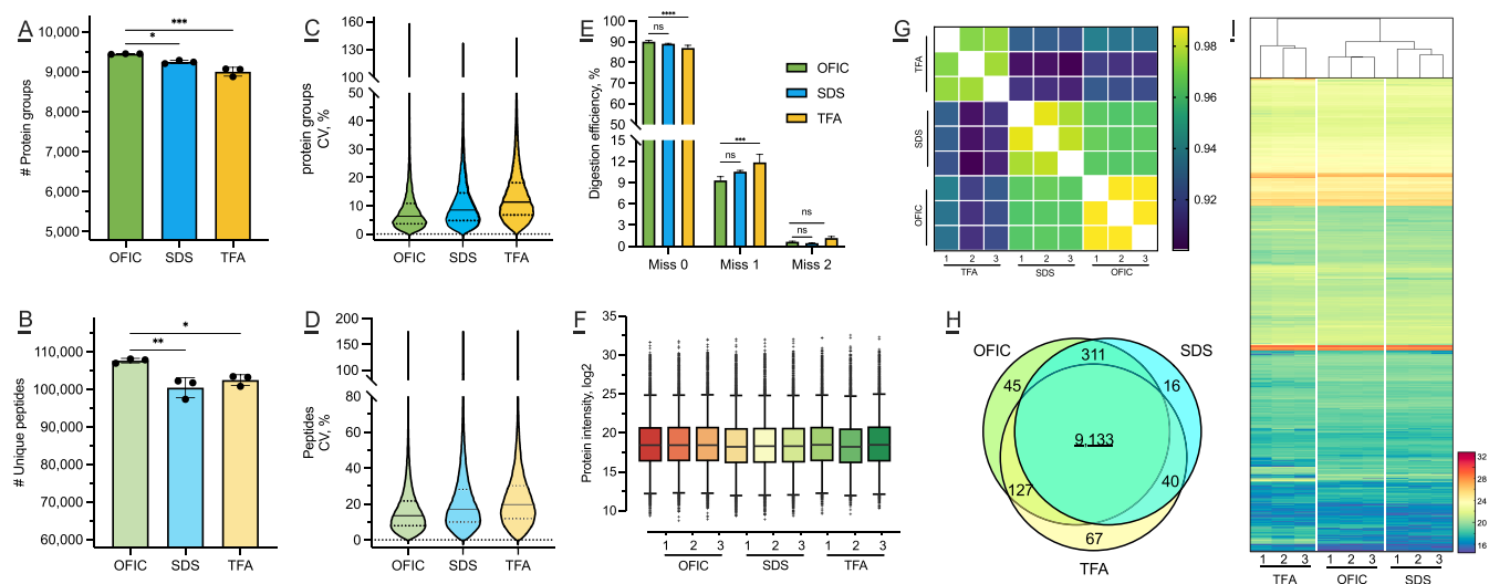
Figure 2. Evaluation of OFIC processing for C. elegans proteome analysis. (A, B) Comparison of the number of proteins and peptides derived from the three processing methods. Three replicate experiments were performed for each method. * p < 0.05 ; ** p < 0.01 ; *** p < 0.001 . (C, D) CV analysis for protein and peptide identifications. (E) Digestion efficiency calculated based on peptide intensity. (F) Box plot of protein intensity. (G) Pearson correlation of replicate experiments between all three methods. (H) Venn diagram of protein identifications. (I) Heatmap of all the proteins quantified by the three methods.
