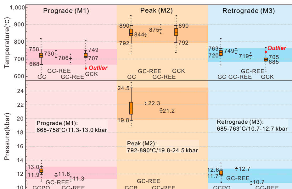
Fig. 3. Plots showing the P-T conditions of garnet clinopyroxenite at different metamorphic stages. The P-T conditions were estimated by various geothermobarometers labeled in the plot. The boxes represent the interquartile range of the dataset of retrieved temperature or pressure. The outliers marked by red dots are far away from other retrieved temperature or pressure values and excluded in the final evaluation of the P-T conditions. The maximum and minimum values of the credible P or T conditions are labeled at the outward extension of the boxes (solid line segment). Dashed lines extending from each P-T box represent the SEs of the employed geothermometers or geobarometers. The geothermobarometers include garnet–clinopyroxene Fe–Mg exchange geothermometer (GC) (56), rare earth element (REE)-based garnet–clinopyroxene thermobarometer (GC-REE) (27), garnet–clinopyroxene Fe–Mg geothermometer (GCK) (57), garnet–clinopyroxene–plagioclase–quartz geobarometer (GCPQ) (58), and garnet–clinopyroxene geobarometer (GCB) (59).
