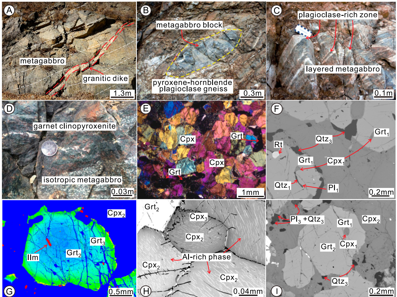
Fig. 2. (A) A granitic dike (outlined by red dashed lines) cross-cuts the internal layering (white dashed lines) of the metagabbro. (B) Metagabbro blocks within the pyroxene-hornblende plagioclase (Pl) gneiss. (C and D) Layered and isotropic metagabbro, which includes garnet (Grt) clinopyroxenite. (E) Clinopyroxene (Cpx) grains in garnet clinopyroxenite have typical triple-junction textures with dihedral angles of \sim 120^\circ , indicating that these grains were in thermodynamic equilibrium during recrystallization. (F) A BSE image showing different stages of quartz (Qtz), Grt, Cpx, and Pl. (G and H) High-contrast BSE images of Grt and Cpx (G is in color scale) displaying zoning texture with the exsolved Al-rich phase on the Cpx surface. Note that the ilmenite (Ilm) within the Grt is likely altered from rutile (Rt) by the metasomatism with retrograde fluid through the cracks within Grt. (I) BSE image showing different stages of Grt and Cpx with small Qtz and Pl around the euhedral garnet.
