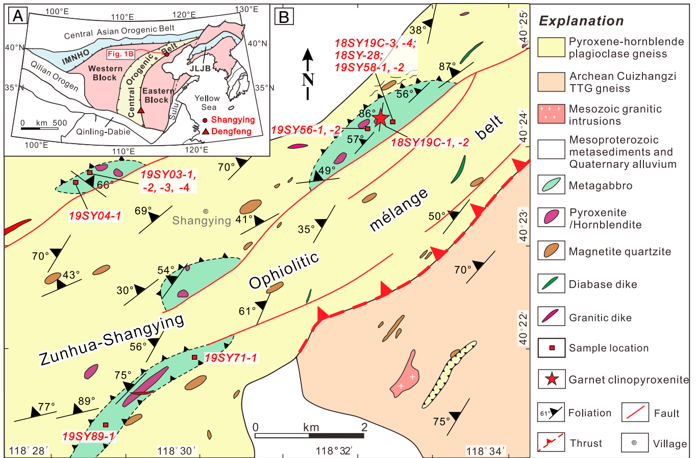
Fig. 1. (A) A geological map showing the tectonic divisions of the NCC (17). The location of the Dengfeng complex and Shangying rock units along the eastern margin of the COB are labeled. Note that the Dengfeng complex has been documented to preserve a late Archean spatially and temporally linked paired metamorphic belt (21). (B) A detailed geological map of Shangying rock units. Note that the garnet clinopyroxenites are enclosed in the metagabbro blocks within the pyroxene-hornblende plagioclase gneiss, which is part of the Archean Zunhua-Shangying ophiolitic mélangé belt ( SI Appendix, Fig. S1B ). IMNHO, Inner Mongolia-Northern Hebei Orogen; JLJB, Jiao-Liao-Ji Belt.
