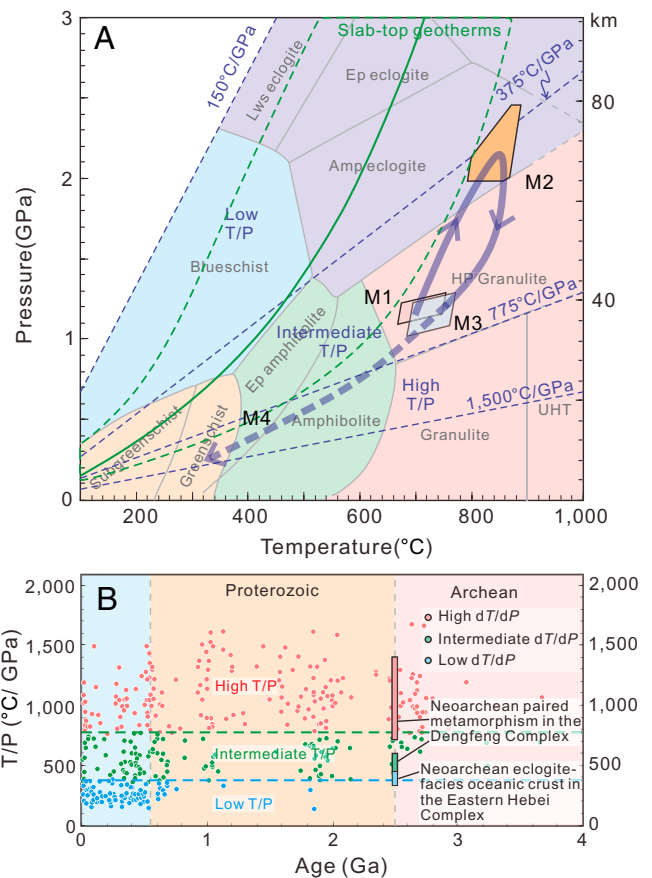
Fig. 4. (A) Retrieved P-T-t path and (B) geothermal gradient (degrees Celsius per gigapascal) of the Shangying garnet clinopyroxenite. The metamorphic facies (60) and the slab-top geotherms of Neoproterozoic to Phanerozoic subduction zones (bounded by the light green dashed lines) (37) are shown. The high, intermediate, and low dT/dP areas delineated by 1,500, 775, 375, and 150°C/GPa are defined based on the global metamorphic P-T dataset (11, 45). dT/dP, differential temperature/differential pressure; UHT, ultra-high temperature. Both the Dengfeng complex and the Eastern Hebei complex are located along the eastern margin of the COB ( SI Appendix, Fig. S1A ), NCC. The Late Archean spatially and temporally linked paired metamorphism documented from the Dengfeng complex (21) and the contemporaneous eclogite-facies oceanic crust in the Eastern Hebei complex (this study), indicate that the modern plate tectonics, characterized by asymmetric and deep subduction, operated at the end of Archean.
