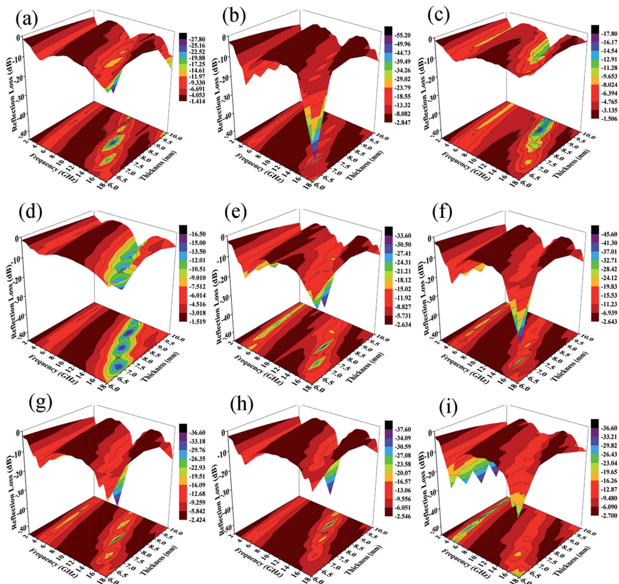
Fig. 12 3D representations of reflection loss of ZNCF (d) and samples of PANI/ZNCF composites T-1 (a); T-2 (b); T-3 (c); D-1 (e); D-2 (f); D-3 (g); D-4 (h); and D-5 (i) in the frequency range of 2–18 GHz.
