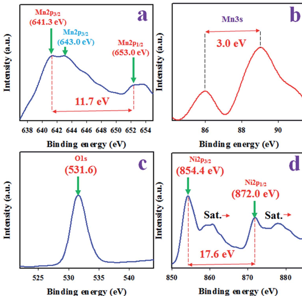
Fig. 1 The XPS analysis of sample Mn 2 O 3 /NiO NPs. (a) Core-level XPS of Mn2p, (b) Mn3s orbit, (c) O1s orbit, and (d) high resolution XPS of Ni2p level.
