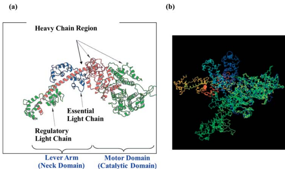
Figure 4. (a) Structure of the myosin head in the rigor state with no nucleotide bound solved by X-ray crystallography ( 4 ). The head consists of a single heavy chain and two light chains, named the essential light chain (ELC) and the regulatory light chain (RLC). It has a motor domain and a neck domain or lever arm. The motor domain is the catalytic domain which has an ATP-binding site and the actin-binding site. The lever arm is a single \alpha -helical with the two light chains (ELC and RLC) bound to it and it connects to the rod portion of the myosin molecules forming the backbone. There are two heads connected to the rod which form a myosin molecule (shown Figure 3a ). (b) Comparison of the myosin head structure from various published crystal structures with different nucleotides bound. All the structures are superimposed at the catalytic motor domain, so that the differences between the models are expressed by the different positions of their lever arms. Green and pointing slightly towards the viewer is the 4 chicken skeletal myosin with no nucleotide bound (i.e. rigor-like); dark blue is the 5 chicken smooth muscle myosin in ADP.AIF 4 form; pale blue is the Lethocerus structure in the relaxed state ( 6 ); orange is the 7 scallop myosin in Mg.ADP.VO 4 form. The view is in the direction such that the actin filament axis is vertical and to the right of the myosin head, with the M-band at the top and Z-band at the bottom.
