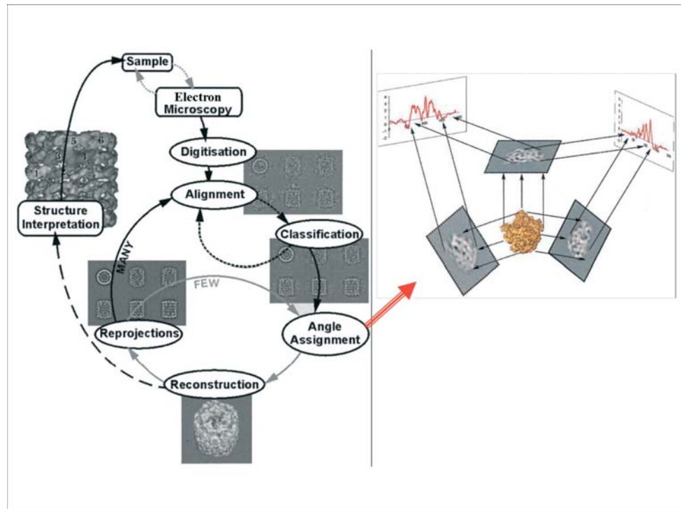
Figure 12. Theory of single particle image analysis using IMAGIC software for 3D image processing ( 74 ).
