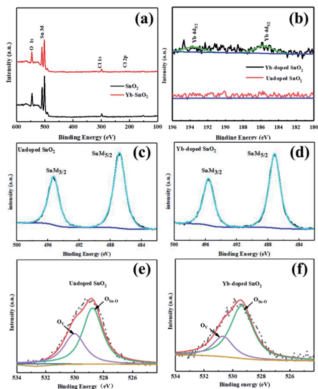
Fig. 3 Full XPS spectra of (a) the undoped SnO 2 film and Yb-doped SnO 2 film, (b) the Yb 4d of the SnO 2 film and Yb-doped SnO 2 film, (c) the Sn 3d of undoped SnO 2 , (d) the Sn 3d of Yb-doped SnO 2 , (e) the O 1s of undoped SnO 2 , and (f) the O 1s of Yb-doped SnO 2 .
