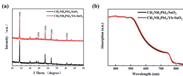
Fig. 2 (a) XRD patterns of perovskite films on pristine SnO 2 and Yb-doped SnO 2 film, (b) the UV-Vis spectra of perovskite films on SnO 2 and Yb-SnO 2 ETLs, respectively.
