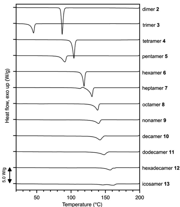
Fig. 4 DSC traces (1 st heating run) of discrete oligomers 2 – 13 at 10\text{ }^\circ\text{C min}^{-1} .
